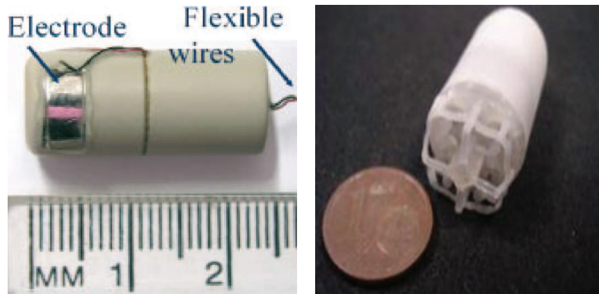
(a) Electric stimulation propulsion robot [80]
