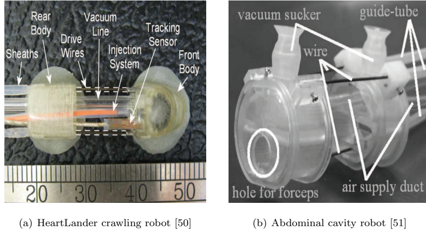
Figure 4: Suction-based in vivo robots
