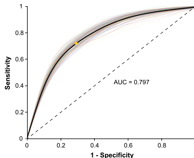
Figure 5. ROC curve for validation results. 200 repeats are plotted in colour, with ROC curve produced from averaging the repeats in black and a marked optimal cut point calculated from Youden's index (yellow dot). Dotted line represents an AUC of 0.50.
