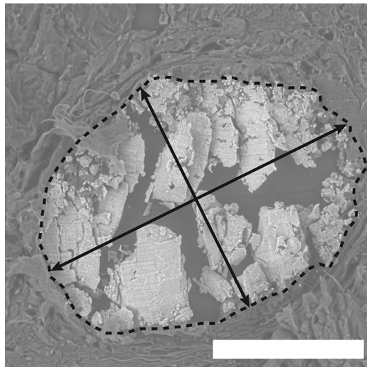
Figure 6. Measurements taken across microcalcifications. XRD data was collected along the longest axis and a perpendicular axis passing through the centre, at 11 \mu\text{m} intervals, marked as double headed black arrows. The longest axis was also measured from SEM images for size analysis. Microcalcification area was measured by outlining each microcalcification (dotted line). The same area was used for EDX analysis. Scale bar = 100 \mu\text{m} .
