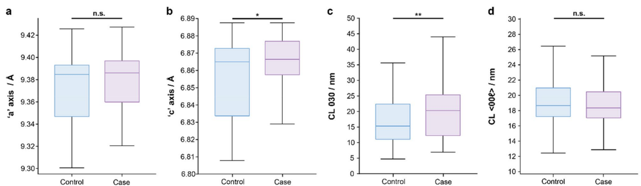
Figure 2. Box plots for HAP parameters determined by XRD. (a) ‘a’ axis lattice parameter, (b) ‘c’ axis lattice parameter, (c) CL for 030, (d) CL for <00c>. n = 179 and 174 for control and case respectively, * p < 0.05 , ** p < 0.01 .
