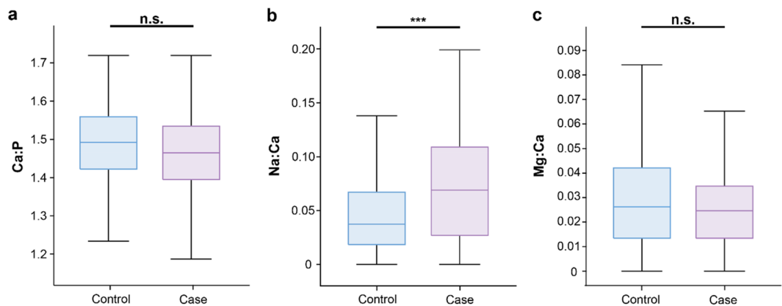
Figure 4. Box plots of EDX analysis of microcalcifications. (a) Ca:P ratio, (b) Na:Ca ratio, (c) Mg:Ca ratio. n = 179 and 174 for control and case respectively, *** p < 0.001 .
