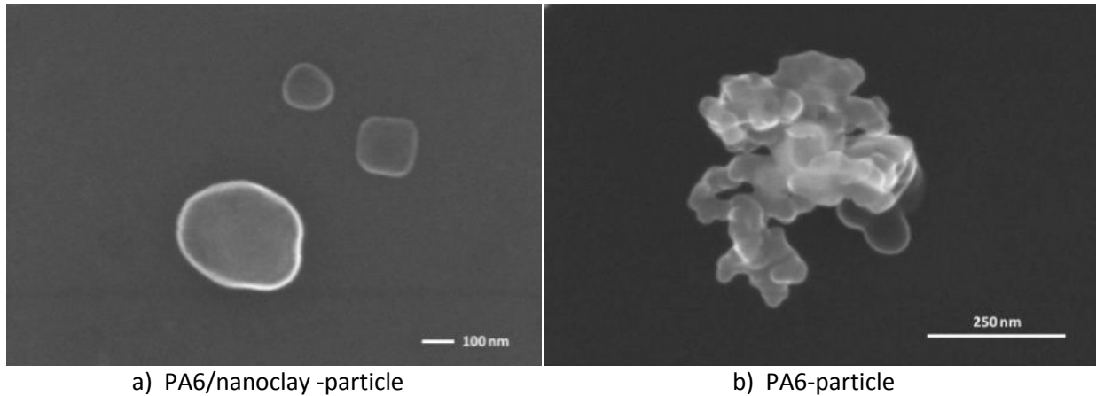
Figure 6 SEM micrographs of a) PA6/nanoclay-particle and b) PA6-particle collected by ESP
