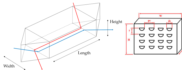
Figure 5. Simplified schematic of the recuperator's geometric parameters.
