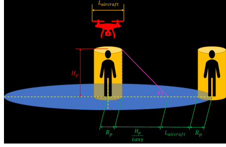
Fig. 5 Radius of the area affected by the fall of the rotor aircraft.
