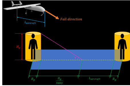
Fig. 3 Length of the area affected by the fall of the fixed-wing aircraft.
