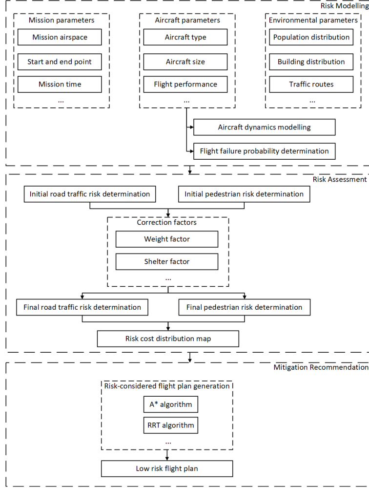
Fig. 1 Structure of the risk assessment approach used in this study.
