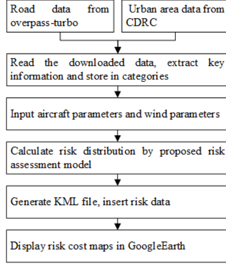
Fig. 8 Flow chart of the risk assessment program working process.
