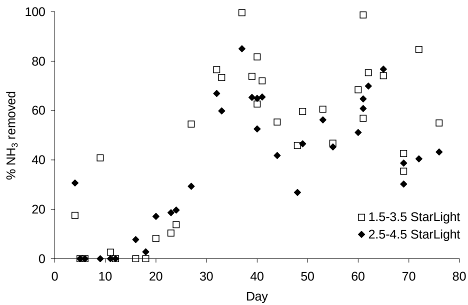
Figure 4: % removal of ammoniacal nitrogen (NH 3 ) during operation
