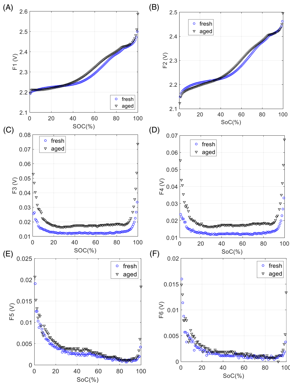
FIGURE 9 Li-S cell charging features recorded at different age levels
