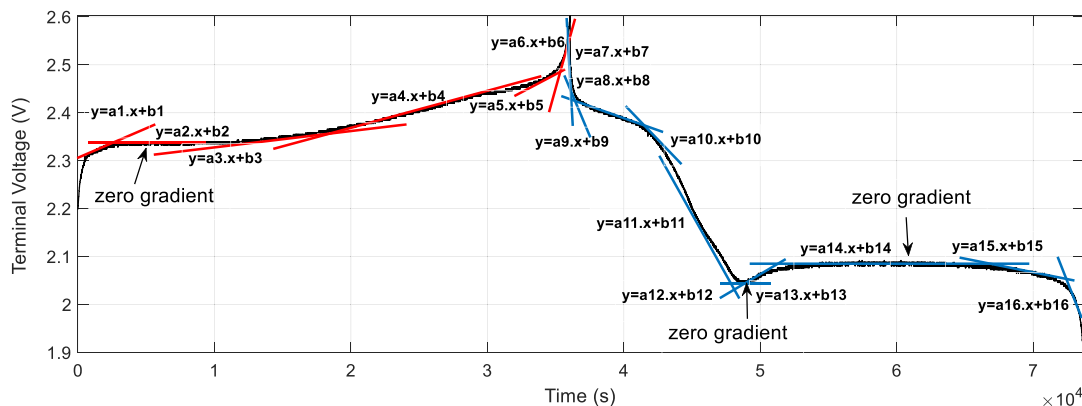
FIGURE 3 Li–S cell charge/discharge voltage curve piecewise linearization
