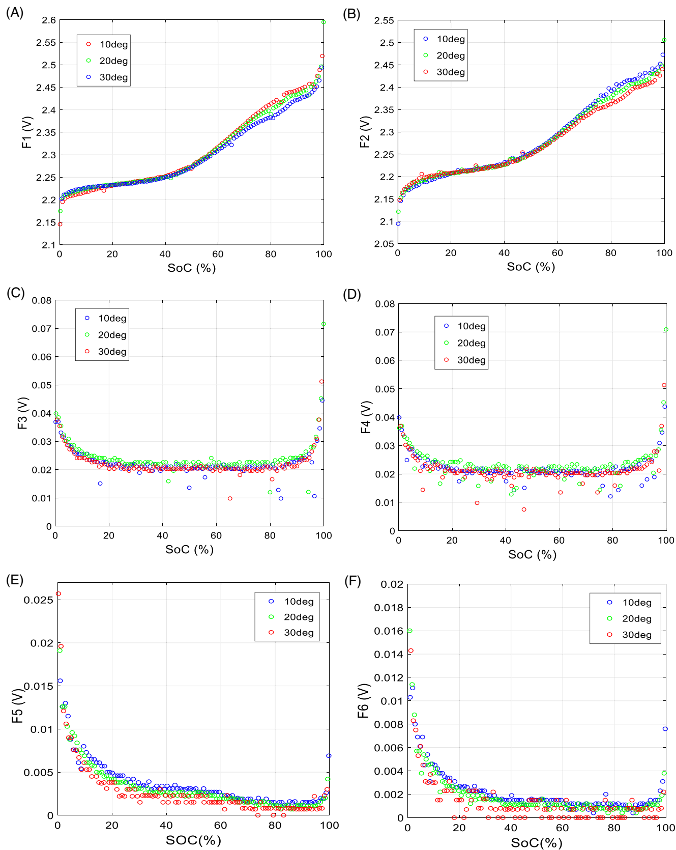
FIGURE 7 Li-S cell instantaneous voltage features (IVF) charging features recorded at different levels of state-of-charge (SoC) and temperature
