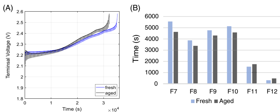
FIGURE 10 The effect of aging on the time-voltage features (TVF) charging features: (A) charging voltage curves, (B) TVF values
