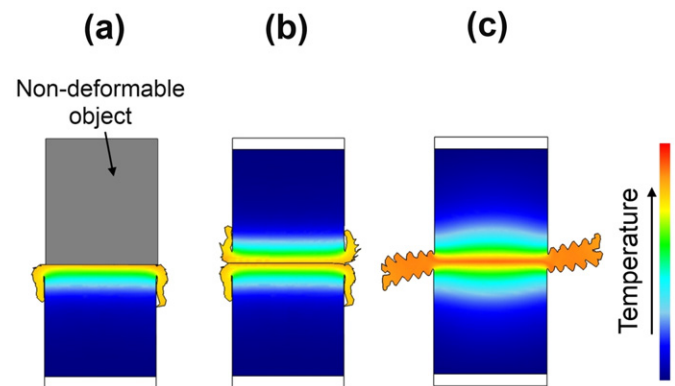
Fig. 3. Modelling approaches: (a) one workpiece, (b) two workpieces (c) a single body representing two workpieces. Adapted from McAndrew et al. [4].
