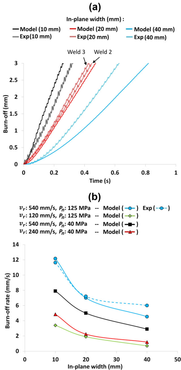
Fig. 12. A comparison of the FEA (Model) and experimental (Exp) results for: (a) the burn-off during phases 2 and 3 vs. time as a function of the in-plane width for an average rubbing velocity of 540 mm/s and a pressure of 125 MPa; and (b) burn-off rate during phase 3 as a function of the in-plane width, average rubbing velocity, v_r , and the normal pressure, P_n .
