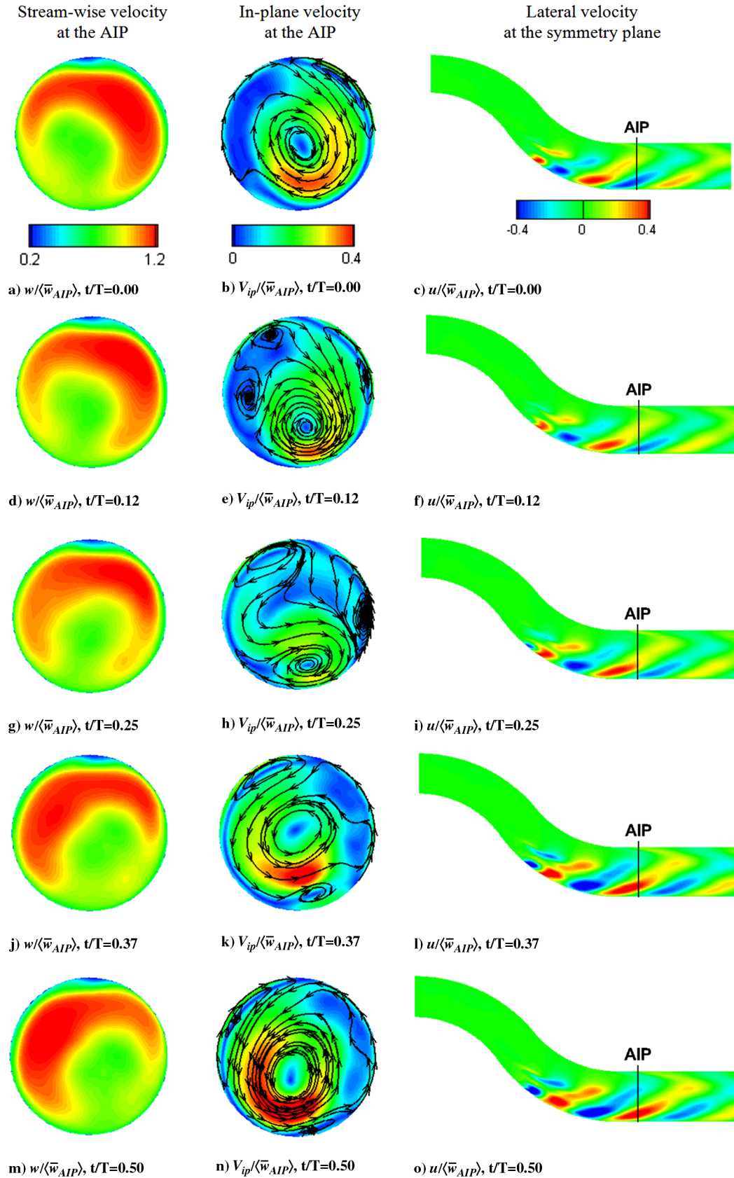
Fig. 13 FVM and SVM of the combined AIP and symmetry plane velocity field POD (DDES, M_{\text{ref}} = 0.27 ).
