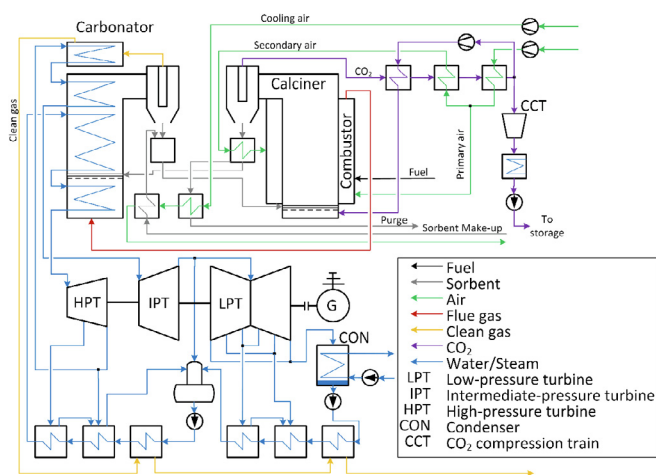
Fig. 2. Scheme of reference case: CaLC with steam cycle.
