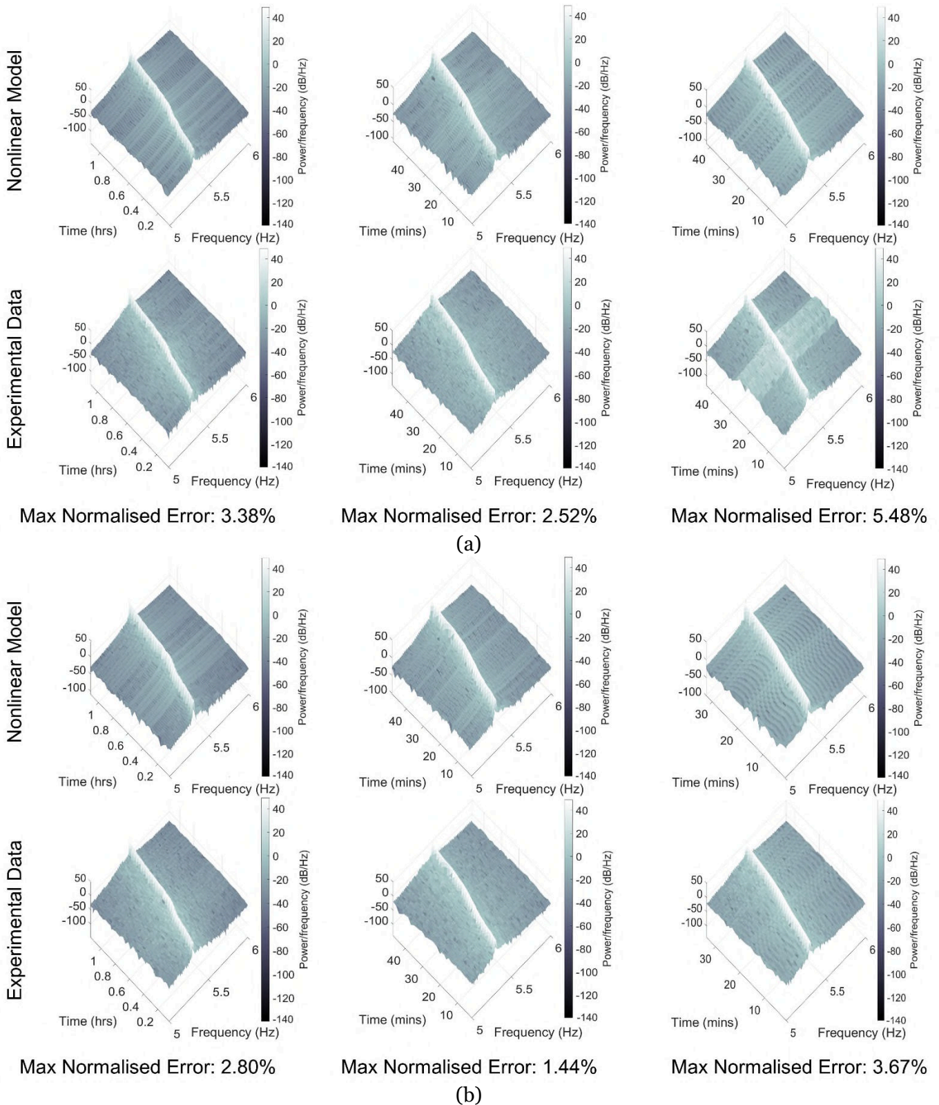
Figure 8. 3-D Waterfall Plots of the recorded output and of the time histories obtained from the nonlinear model. (a) Unloaded case, (b) Sensor-loaded case. The recording for the largest input suffered from clipping for the unloaded case.
