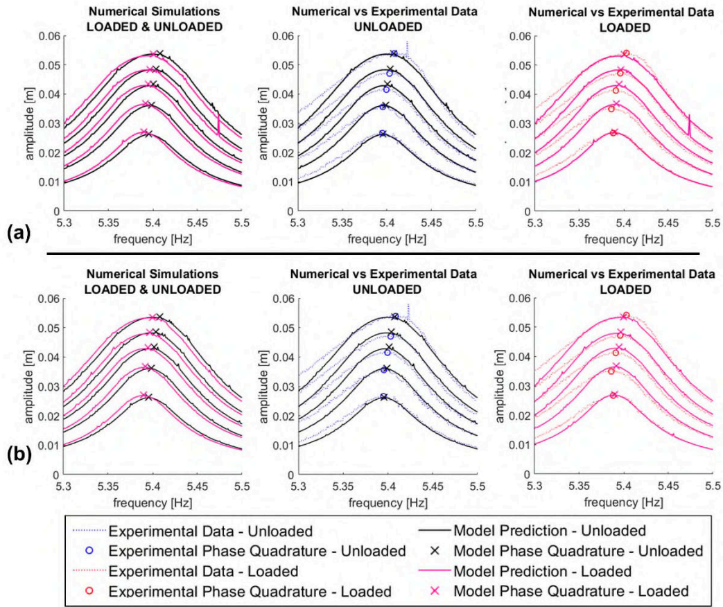
Figure 7. Modulation Equation results: (a) optimised integer values of \eta and \rho (b) optimised non-integer values of \eta and \rho .
