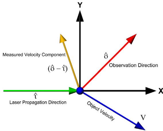
Figure 1. The relationship of laser illumination direction and observation direction to the measured velocity component determined from the Doppler equation.
