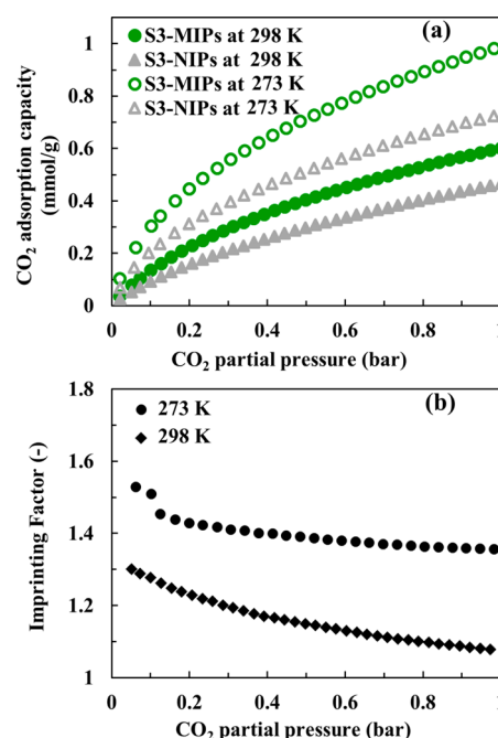
Figure 5. (a) Comparison of \text{CO}_2 adsorption isotherms of S3-MIPs and S3-NIPs at 273 and 298\text{ K} ; (b) The imprinting factors of S3 at 273 and 298\text{ K} at \text{CO}_2 partial pressures up to 1\text{ bar} .
