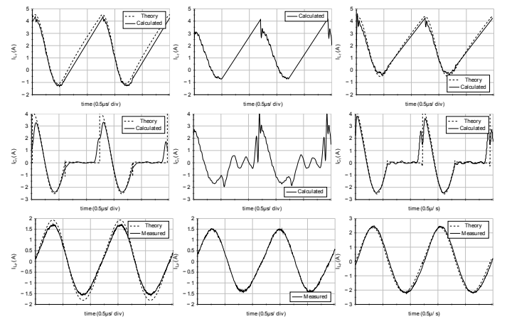
Fig. 9. Current waveforms of the implemented WPT system at different coupling coefficients demonstrating the proposed tuning method. The waveforms represent the DC-feed inductor's current I_{Lf} , the shunt capacitor's current I_{C1} and the primary coil's current I_{LP} .
