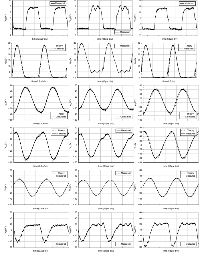
Fig. 8. Voltage waveforms of the implemented WPT system at different coupling coefficients demonstrating the proposed tuning method. The waveforms represent the MOSFET's gate driving signal V_{GS} , the MOSFET's drain voltage V_{DS} , the voltage across the series capacitor V_{C2} , the voltage across the primary coil V_{LP} , the output voltage at the load V_R and the voltage developed across the control windings of one of the saturable reactors V_{sat} .
