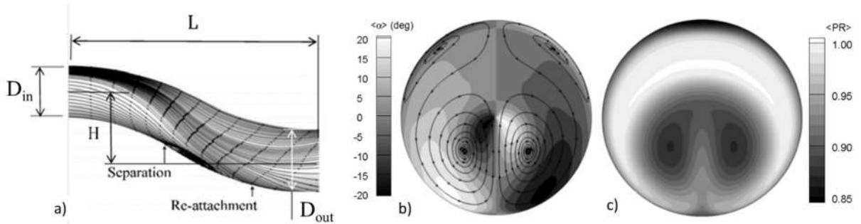
Fig. 1 RANS predicted flow field. (a): surface streamlines (b): swirl angle (c): AIP total pressure ratio [7].
