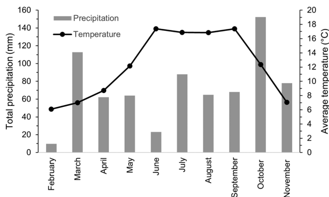
FIGURE 1 Monthly total precipitation and average temperature during the experiment.
