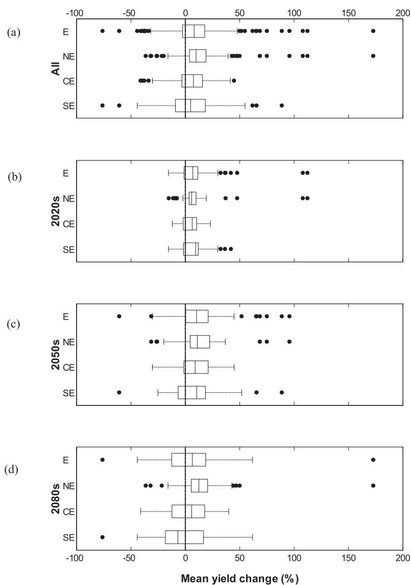
Figure 4. Box and whisker plots showing the variation in projected change in average yield (%) for (a) all observations ( n = 729 ) by region in Europe and for selected time slices including the 2020s (b), the 2050s (c) and the 2080s (d).
