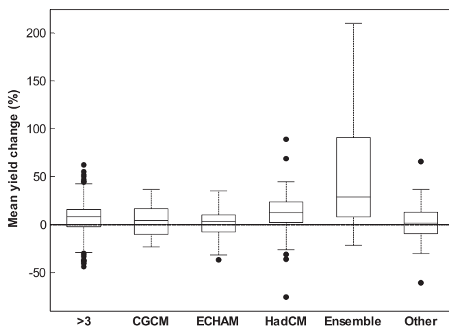
Figure 5. Box and whisker plot showing projected changes in average yield (%) for all crops using either a single, ensemble or group (>3) of GCM climate models.
