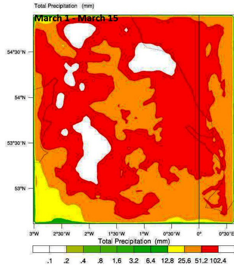
Figure 10: The accumulated precipitation results obtained from WRF with WRF SM3 and BMJ schemes from 1 st March to 14 th march
