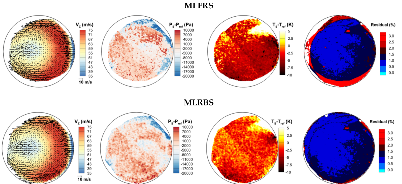
Fig. 8. Comparison of the flow fields derived with MLFRS and MLRBS methods at the S-duct outlet plane for inlet Mach = 0.27. In-plane velocity vectors on V_z component are limited to a 4.5 mm spacing to improve clarity.
