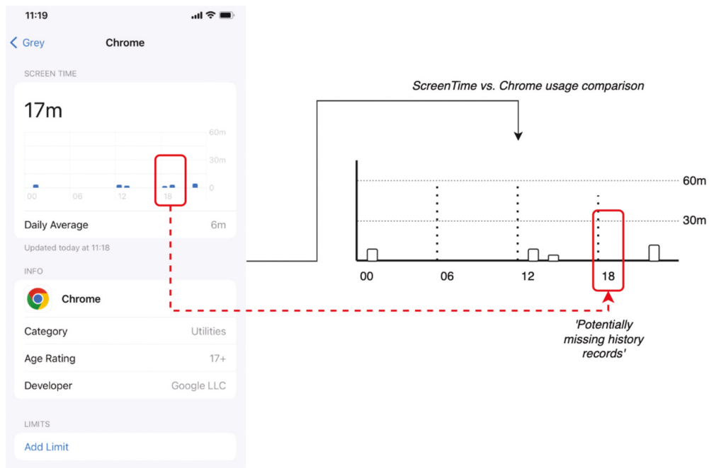
Figure 7. A comparison between activity logged on ScreenTime for Chrome vs. Chrome's internet history records showing private browsing behaviour.
