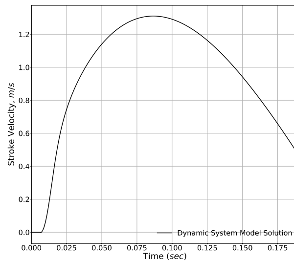
Figure 2. Shock absorber stroke velocity profile from a dynamic system model simulating a drop test used to choose a suitable inlet velocity value in the LES study.
