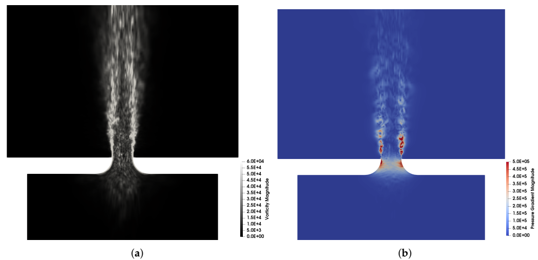
Figure 8. Contours of the vorticity magnitude (calculated using the instantaneous velocity field) showing the unsteadiness not only in the vicinity of the orifice in the shear layers as expected but also in the central potential flow region of the jet. Contours of the pressure gradient magnitude are also plotted to identify regions susceptible to the appearance of cavitation bubbles, which could lead to high transient stresses on nearby surfaces when these bubbles collapse. (a) Vorticity magnitude contours. (b) Pressure gradient contours.
