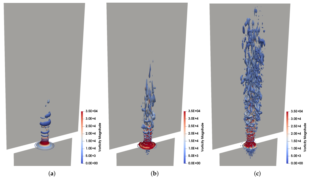
Figure 4. Q Criterion iso-surfaces used to visualise the development of coherent structures in the vicinity of the orifice and in the mixing layer. The initial laminar rings capture the transitional phase as the flow accelerates from a stationary state through the orifice, leading to the appearance of these axisymmetric Kelvin–Helmholtz type rollers, which then develop secondary instabilities as they are convected in the streamwise direction until they breakdown further downstream forming smaller three dimensional turbulent structures. (a) Initial laminar instabilities. (b) Developing turbulent flow. (c) Developed turbulent shear layer.
