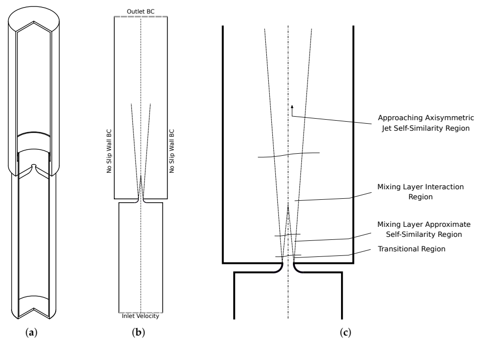
Figure 1. Shock absorber geometry and some setup details (a) Schematic view of the simplified shock absorber geometry; (b) The computational domain with the applied boundary conditions; (c) Axisymmetric shear layer development regions, following Bradshaw et al. [11].
