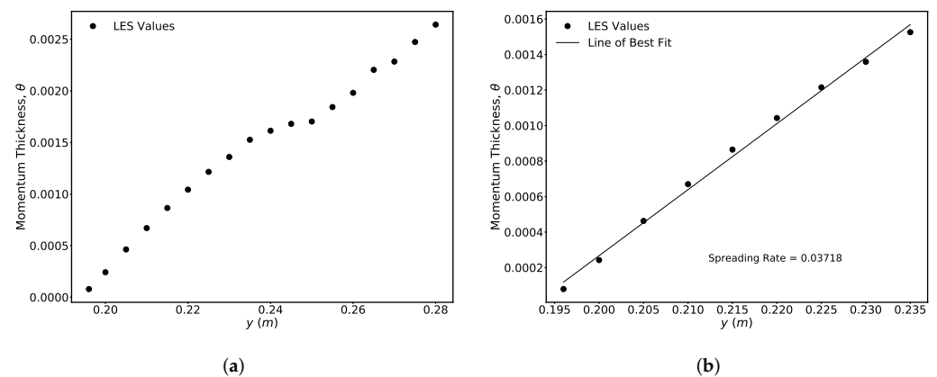
Figure 7. Mixing layer spreading rate estimation based on the momentum thickness growth plotted over a streamwise distance covering the initial linear region and extending into the region where three-dimensional effects are expected to become significant as the axisymmetric shear layer transitions into an axisymmetric jet. In (b), a line of best fit is inserted through the strongly linear initial mixing layer phase up to approximately Y/D_{orifice} \approx 5 , yielding the spreading rate SR_\theta = 0.03718 . (a) Points up to Y/D_{orifice} \approx 9 . (b) Points up to Y/D_{orifice} \approx 5 .
