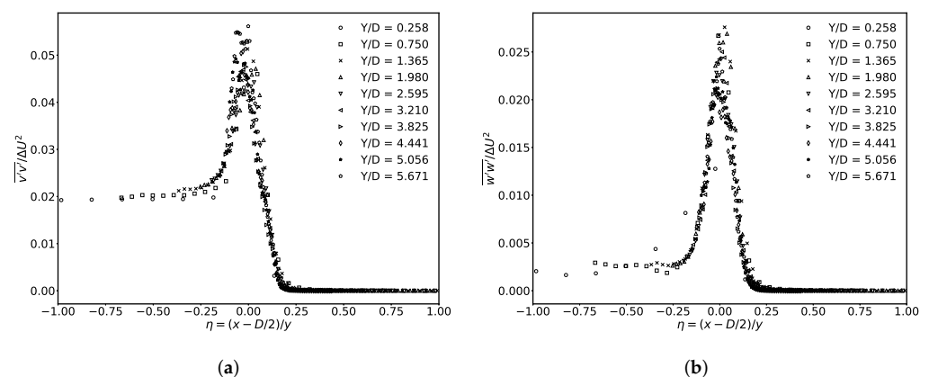
Figure 10. Self-similarity plots of the mixing layer's Reynolds stress profiles, \overline{v'v'} and \overline{w'w'} confirm the presence of relatively high turbulent intensity values on the high velocity potential core side of the profiles. (a) Streamwise Reynolds stress, \overline{v'v'} . (b) Cross-stream Reynolds stress, \overline{w'w'} .
