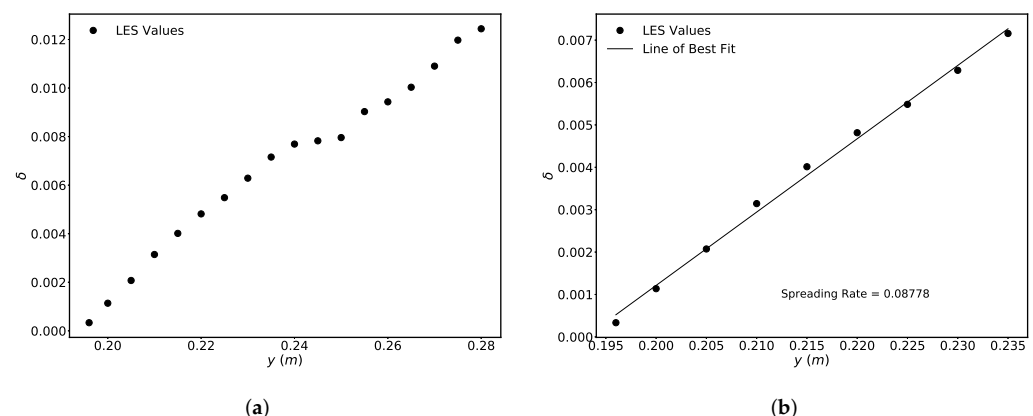
Figure 6. Mixing layer spreading rate estimation based on the expansion of velocity fraction lines plotted over a streamwise distance covering the initial linear region and well into the region where three-dimensional effects are expected to become significant as the axisymmetric shear layer transitions into an axisymmetric jet. In (b), a line of best fit is inserted through the strongly linear initial mixing layer phase up to approximately Y/D_{orifice} \approx 5 , yielding the spreading rate SR_\delta = 0.0878 . (a) Points up to Y/D_{orifice} \approx 9 . (b) Points up to Y/D_{orifice} \approx 5 .
