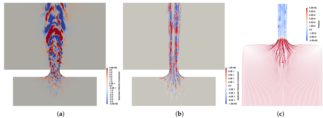
Figure 9. Contours of the spanwise velocity component can be used to highlight the development of instabilities and turbulent flow in the shock absorber as this component should remain negligible, by symmetry, unless some form of three-dimensional flow structures are detected. The field development here is consistent with the vorticity magnitude contours seen in Figure 8. Traces of the streamlines are plotted to visualise the unsteadiness upstream of the orifice and show the potential cause, which is the influence of the flow turning at the orifice boundary that creates a converging flow around the axis of symmetry rotating the flow from the radial to the streamwise direction. (a) Spanwise velocity component. (b) Streamlines coloured by spanwise velocity component. (c) Streamlines showing disturbances upstream of the orifice, coloured by pressure.
