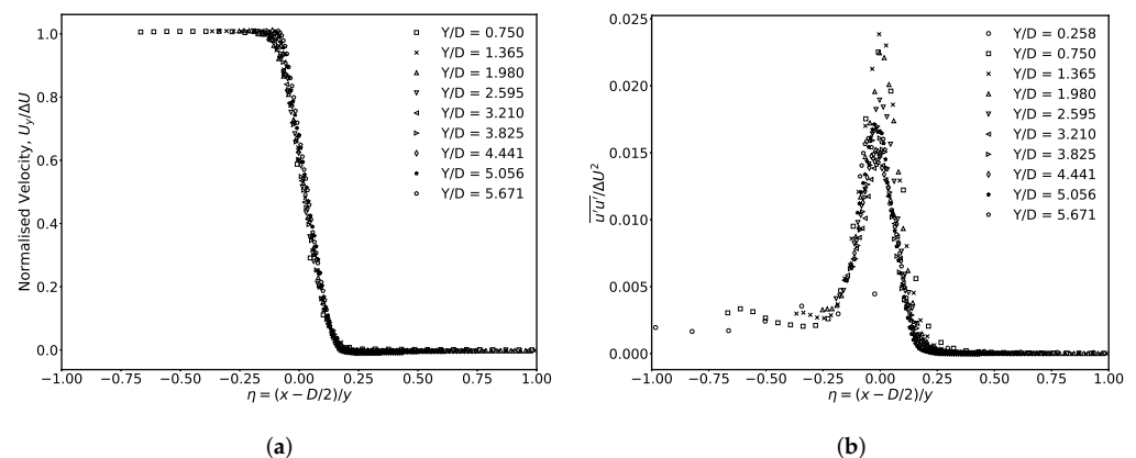
Figure 5. Self-similarity is detected in the shear layer development as the velocity profiles and Reynolds stress profiles, \overline{u'u'} , are seen to collapse on a single line after appropriate scaling. The turbulent Reynolds stress is observed to require longer streamwise development than velocity to reach this state. (a) Streamwise velocity. (b) Cross-stream Reynolds stress, \overline{u'u'} .
