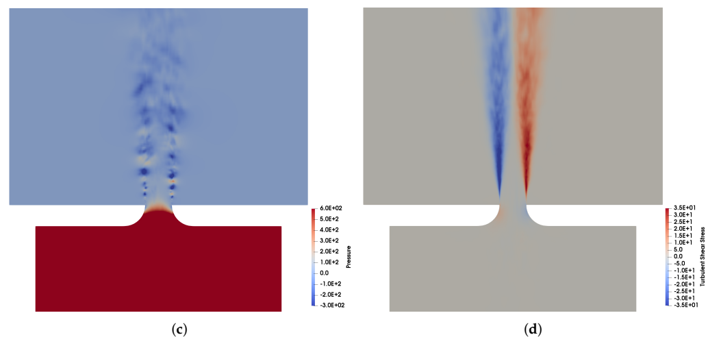
Figure 3. Field contours illustrating the shear layer development through the orifice with the expected turbulent scales appearing in the instantaneous velocity contours while the smoother time-averaged contours show the growth of the shear layers on moving downstream. Pressure fluctuations appear periodically as a result of the developing shear layer instabilities near the orifice exit, while the turbulent shear stress contours help identify regions of high turbulent mixing. (a) Instantaneous Velocity. (b) Mean Velocity. (c) Static Pressure. (d) Turbulence Shear Stress.
