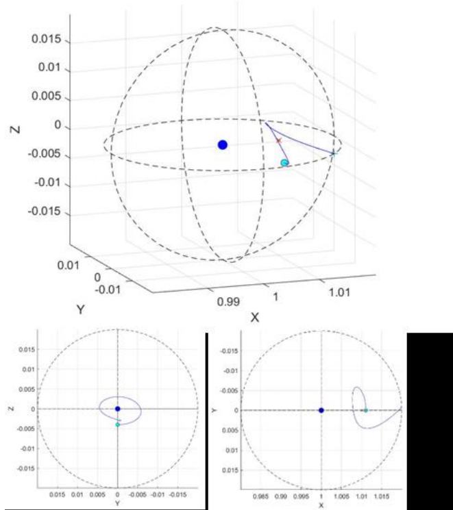
Figure 16. Example of direct escape trajectory. The blue line shows the trajectory. The Earth is plotted as a blue circle, on the centre of the control radius, SE L2 point as a red cross. And the control sphere is illustrated in black dashed line. The image is displayed from three standpoints: perspective view, YZ plane and XY plane.
