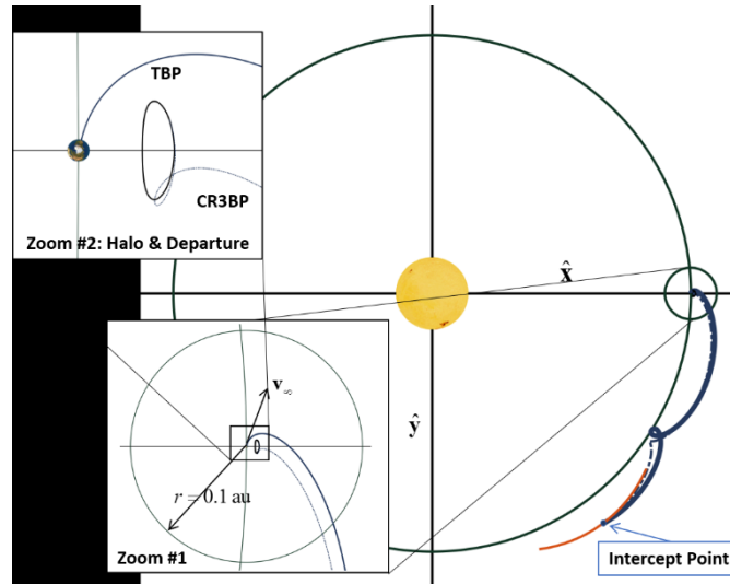
Figure 5. Example of Comet Intercept Transfer (same as Figure 4) in Synodic, or rotating, reference frame. Zoom #1 and #2 represent the Earth escape phase. Earth and Sun are plotted 30 times larger than they should be.
