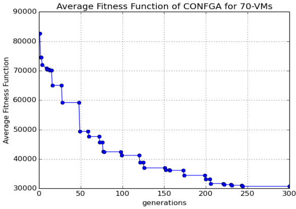
Figure 4: Average CONFGA Performance with 70VMs Problem Instance
