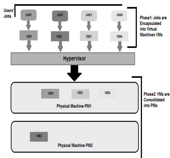
Figure 1: Resource allocation phases in Cloud computing
