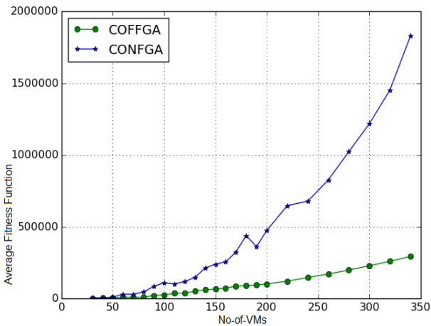
Figure 5: Comparison between COFFGA and CONFGA in terms of average fitness function for 26 problem instances over 8 runs
