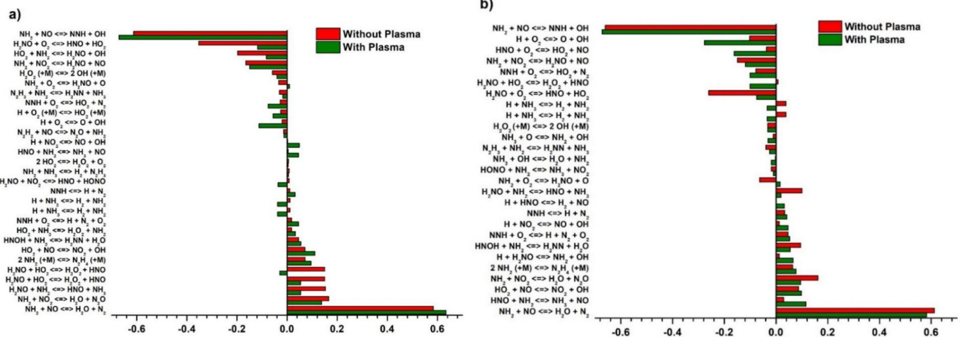
Fig. 12. IDT Sensitivity analysis for \text{NH}_3/\text{air} mixture without and with 20 pulses of NSPD at p = 1 atm, \Phi = 1 , E/N = 180 Td, and PRF = 50 KHz. a) 850 K and b) 1050 K.
