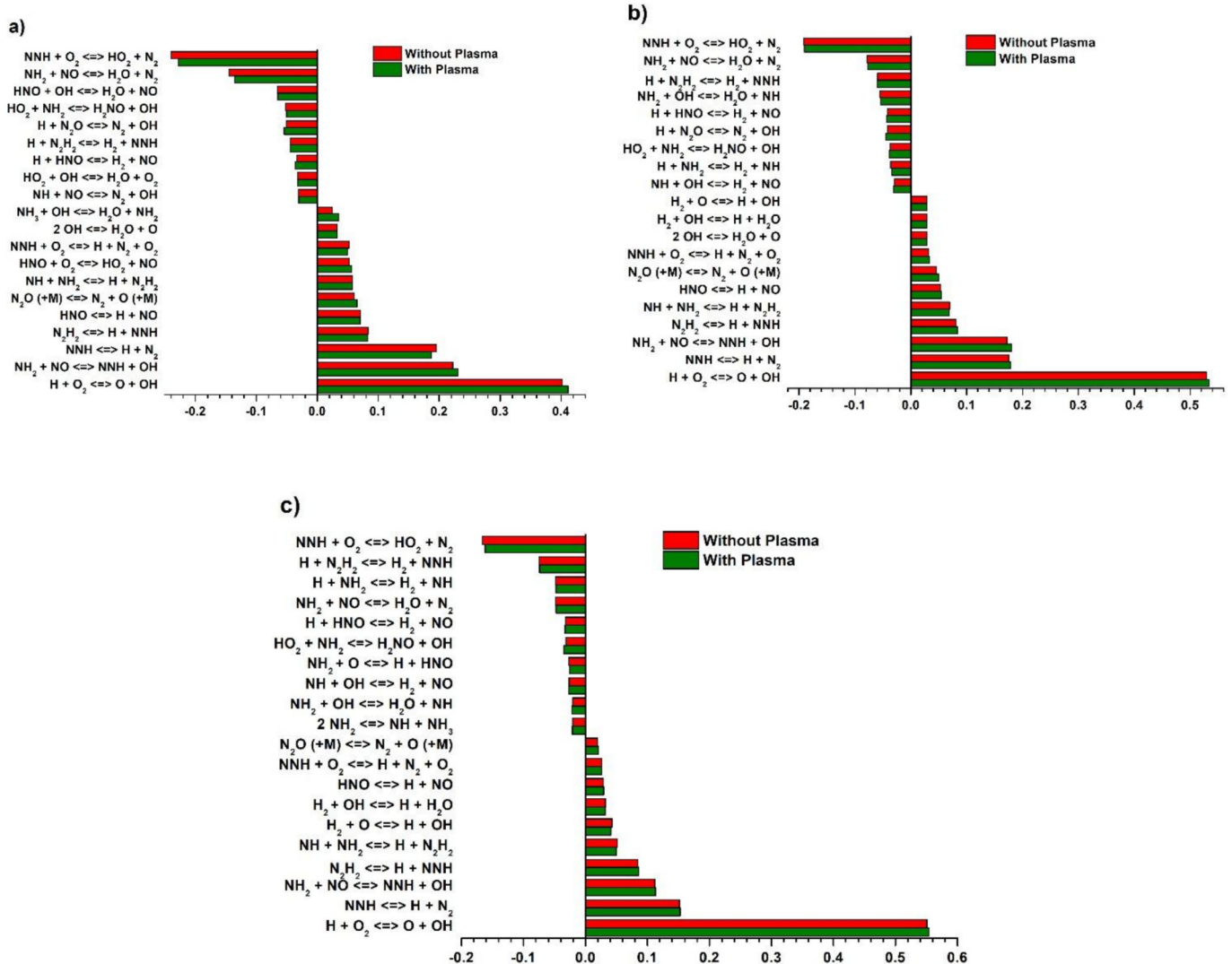
Fig. 14. Sensitivity analysis for LFS of \text{NH}_3/\text{air} without and with 20 pulses of NSPD at T = 450 K, p = 1 atm, E/N = 180 Td, and \text{PRF} = 50 KHz. a) \Phi = 0.8 . b) \Phi = 1.0 and c) \Phi = 1.2 .
