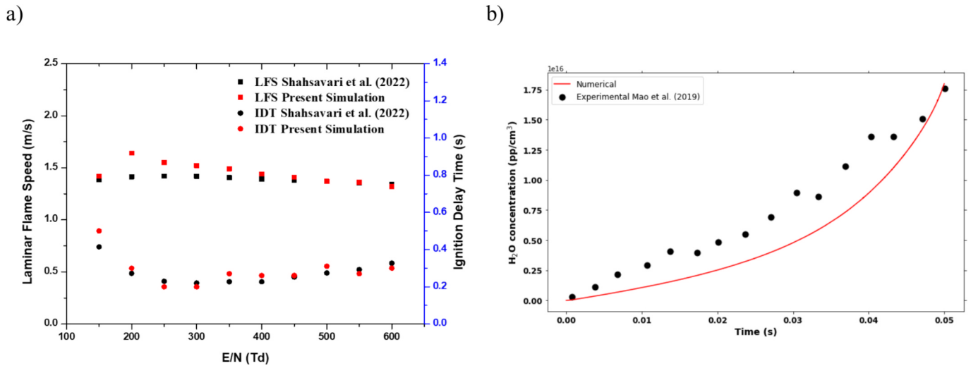
Fig. 5. A) plasma-assisted \text{NH}_3/\text{O}_2/\text{N}_2 combustion for \phi = 1 , T_{\text{in}} = 850 K with PRF = 50 kHz and E_p = 5 mJ/cm 3 IDT and LFS. b) \text{H}_2\text{O} number density with model prediction during and after the 1500 pulse, 30 kHz nanosecond plasma in burst modes for a 0.1667 \text{H}_2 /0.0833 \text{O}_2 /0.75 He mixture at 60 Torr.
