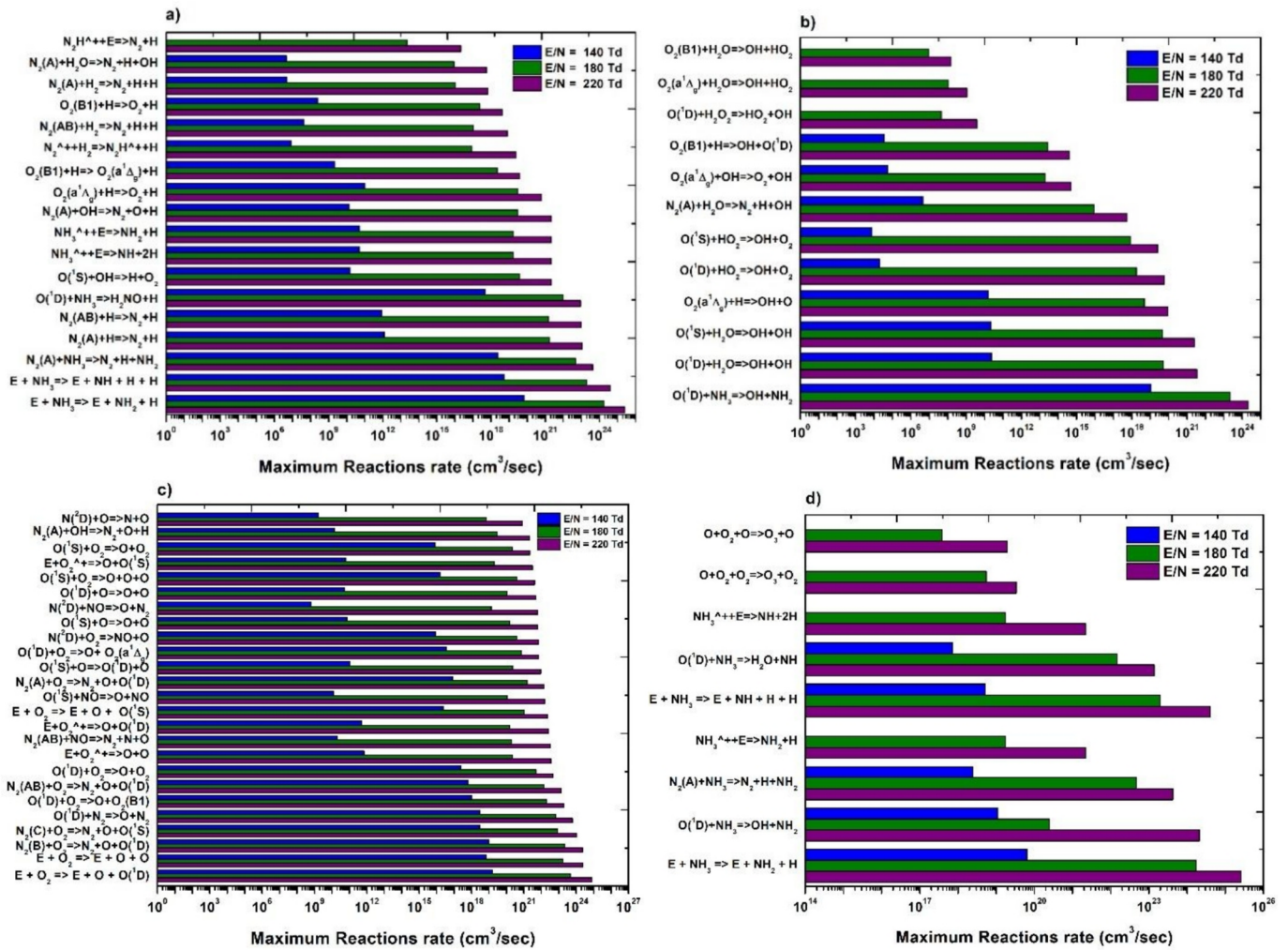
Fig. 8. The maximum reaction rate for the important reactions that participate in the production of a) H. b) OH. c) O, and d) \text{NH}_2 , \text{NH} , \text{O}_3 during 20 pulses of NSPD at p = 1 atm, T = 850 K, and \text{PRF} = 50 kHz.
