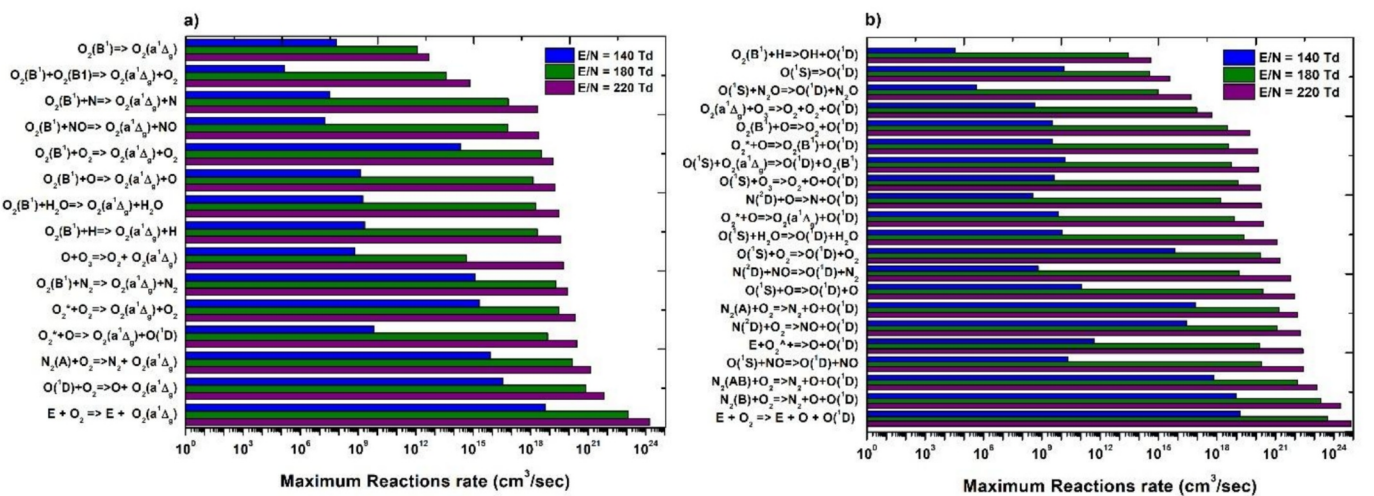
Fig. 9. The maximum reaction rate for the important reactions that participate in the production of a) \text{O}_2(\text{a}^1\Delta_g) and b) \text{O}(\text{D}) during 20 pulses of NSPD at p = 1 atm, T = 850 K, and \text{PRF} = 50 kHz.
