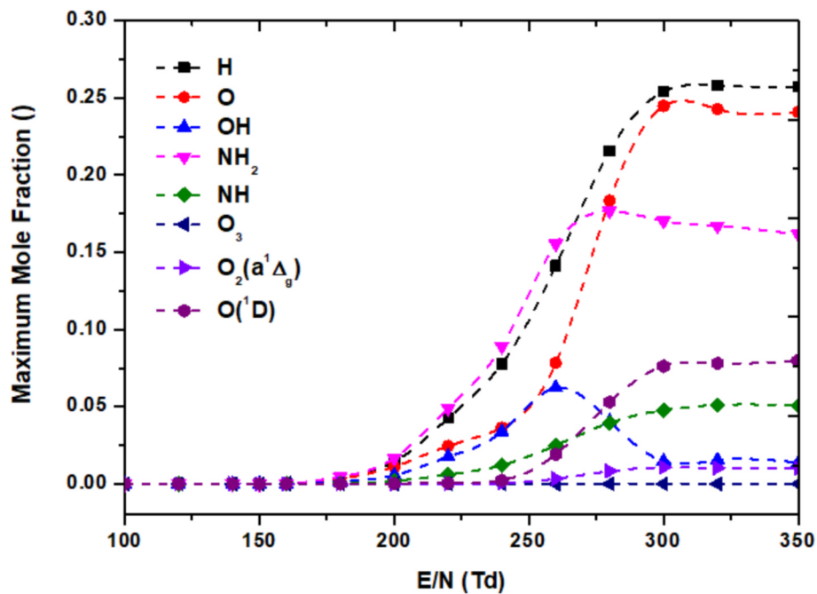
Fig. 6. Maximum molar fractions of active and excited species in 20 pulses of NSPD in an \text{NH}_3 /air mixture at T = 850 K, p = 1 atm, \Phi = 1.0 with PRF = 50 kHz.
