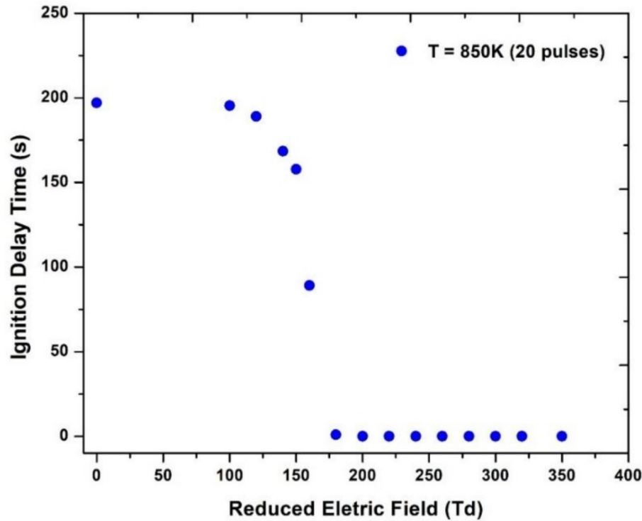
Fig. 7. Effect of E/N on IDT for an \text{NH}_3/\text{air} mixture at T = 850 \text{ K} , p = 1 \text{ atm} , and \Phi = 1.0 , with 20 pulses of NSPD at a PRF of 50 kHz.
