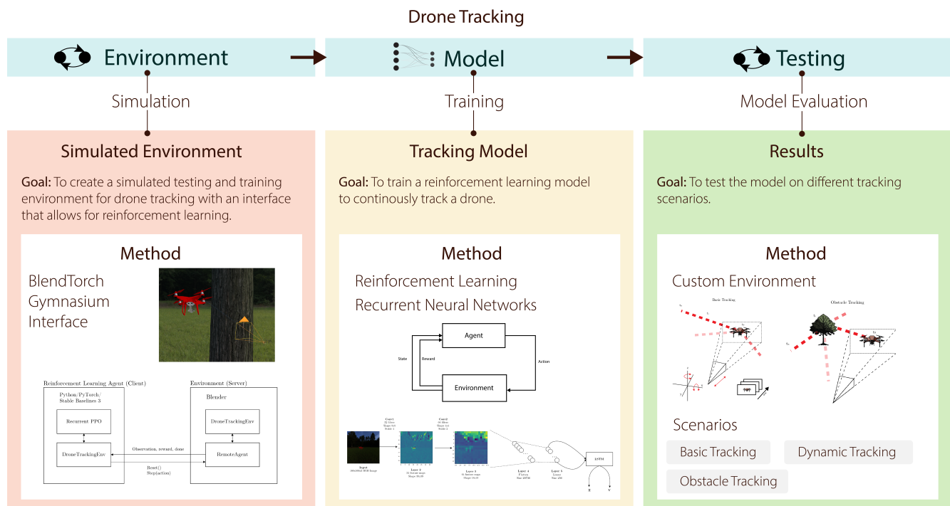
Figure 1. The holistic approach shown in this paper, split into three main sections: environment, the model, and testing. The environment is the simulation of the pan–tilt–zoom (PTZ) camera and the flying drone. This is carried out in Blender, combined with the Blendtorch Gymnasium Interface. The model used to control the PTZ is trained using reinforcement learning (RL). The model is trained and evaluated in multiple environments: Basic Tracking, Dynamic Tracking, and Obstacle Tracking.
