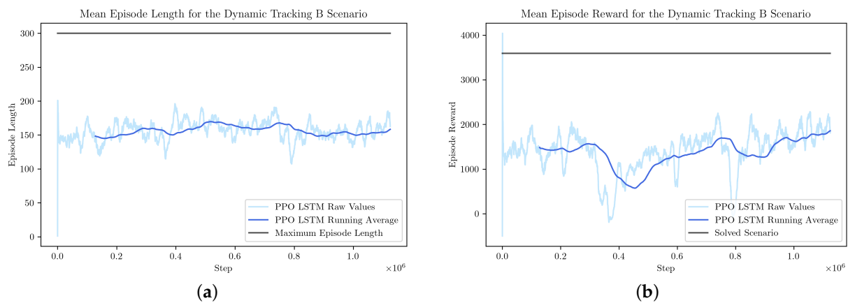
Figure 14. Average episode length (a) and average episode reward (b) for the dynamic tracking B scenario.
