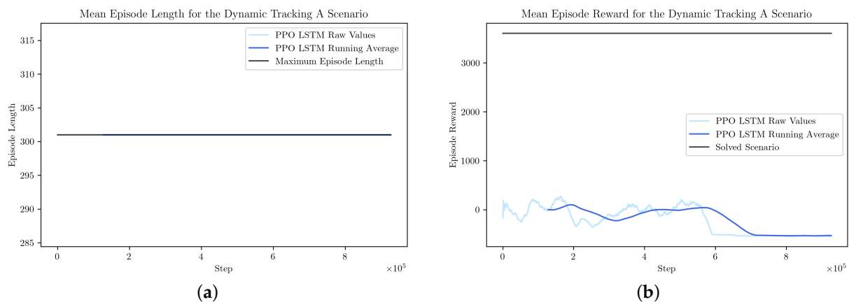
Figure 12. Average episode length (a) and average episode reward (b) for the dynamic tracking A scenario.
