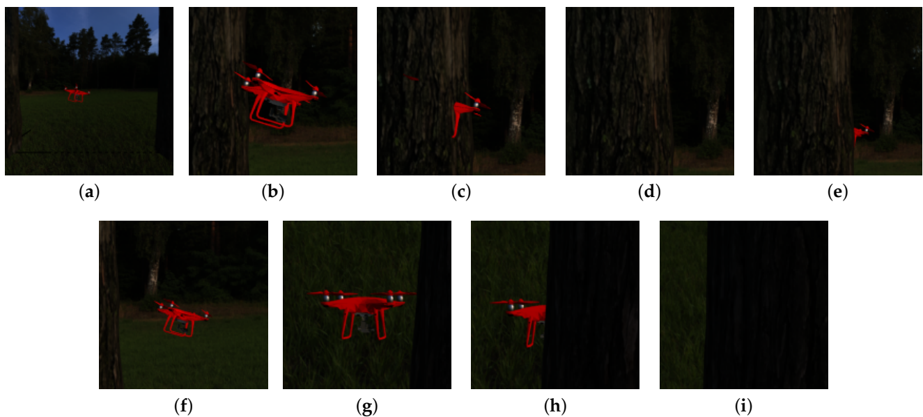
Figure 17. Viewport from the camera at (a) frame 1, (b) frame 100, (c) frame 128, (d) frame 200, (e) frame 275, (f) frame 300, (g) frame 400, (h) frame 408, (i) frame 428 during an episode of the Obstacle Tracking scenario. The agent correctly tracks the drone for 428 frames in this episode, although loses sight of the drone as it gets lost behind another obstacle and does not reach 450 frames.
