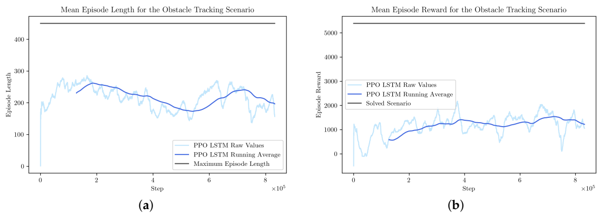
Figure 16. Average episode length (a) and average episode reward (b) for the obstacle tracking scenario.
