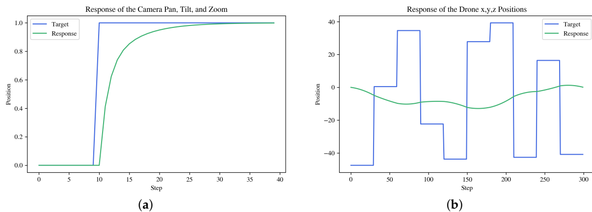
Figure 6. The input and response of the systems for pan, tilt, and zoom controls for the camera (a), and for x, y, z, target positions of the drone (b).
