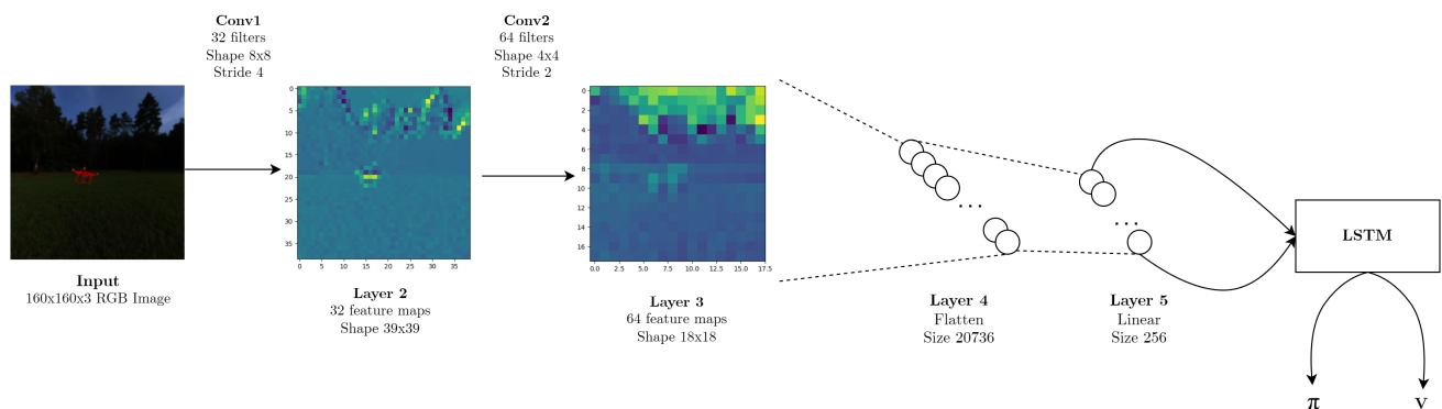
Figure 8. Architecture of the neural network. The input is an RGB image received from the environment. It is passed through an encoder which consists of two convolutional layers. The features from layer 3 are flattened in layer 4 and outputted to 256 features in layer 5. These features are input into an LSTM layer and an actor–critic multilayer perceptron which predicts the value and the policy.
