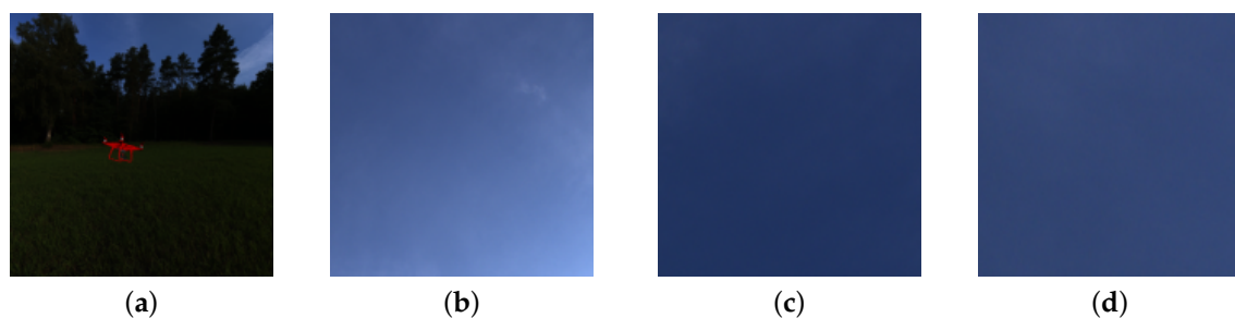
Figure 13. Viewport from the camera at (a) frame 1, (b) frame 75, (c) frame 225, (d) frame 300 during an episode of the Dynamic Tracking A scenario. The agent fails to learn to track the drone in this episode and instead turns around in circles.
