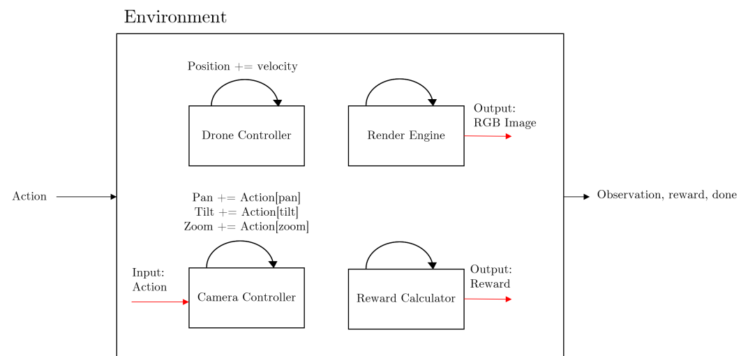
Figure 3. Environment step. At every step, an action is input into the environment. The camera controller takes the action and updates the camera’s pan–tilt–zoom (PTZ) parameters. The drone controller updates the position of the drone. The render engine renders the scene and outputs an RGB image (which is the observation). The reward calculator finds the area occupied by the drone in the image and outputs the reward/termination based on this.
