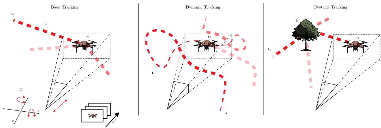
Figure 4. Different scenarios used to train and evaluate the RL agent. Basic tracking, dynamic tracking, and obstacle tracking. In basic tracking, the drone is assigned a random velocity at the start of the scenario and the velocity does not change until the end or termination. In dynamic tracking, the drone changes a waypoint every 30 steps. The drone is modelled as a second-order dynamic system, hence the acceleration is variable. In obstacle tracking, the drone flies behind an obstacle and then is assigned a random velocity when behind the obstacle.
