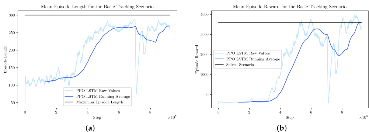
Figure 9. Average episode length (a) and average episode reward (b) for the Basic Tracking scenario.
