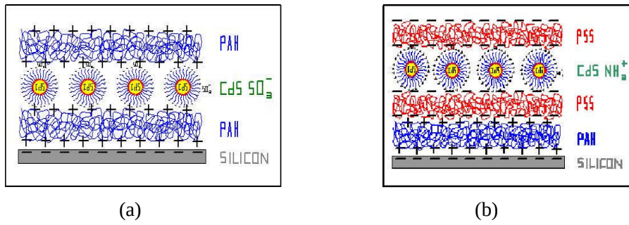
Figure 1. Deposition of colloid nanoparticles CdS-SO 3 - (a) and CdS-NH 2 + (b).
