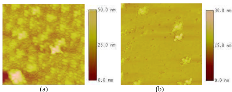
Figure 7. Tapping mode AFM images (1 \mu\text{m} in size) of CdS-NH 2 + layers deposited from colloid solutions diluted in 100 times (a) and 500 times (b).
