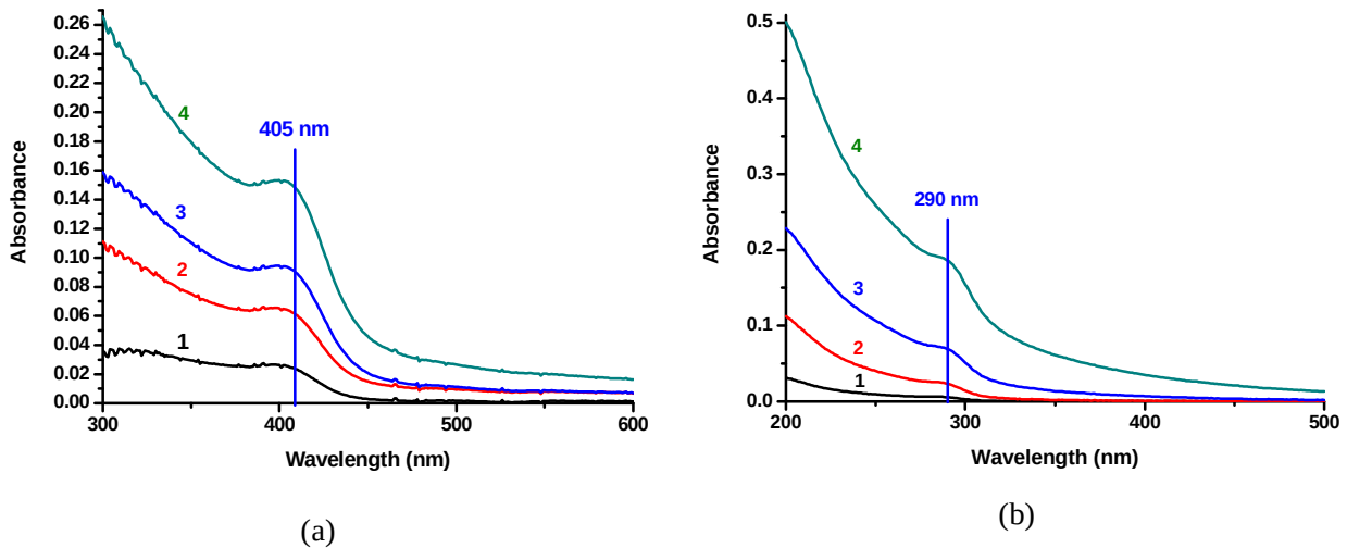
Figure 2. UV-vis absorption spectra of PAH/ \text{CdS-SO}_3^- film (a) and PAH/ \text{ZnS-SO}_3^- film (b). The numbers near respective spectra correspond to the number of polyelectrolyte/nanoparticle bilayers.
