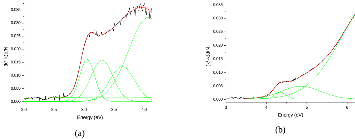
Figure 3. Gaussian fitting of the spectra of the first layer of CdS-SO 3 - (a) and the first layer of ZnS-SO 3 - (b).
