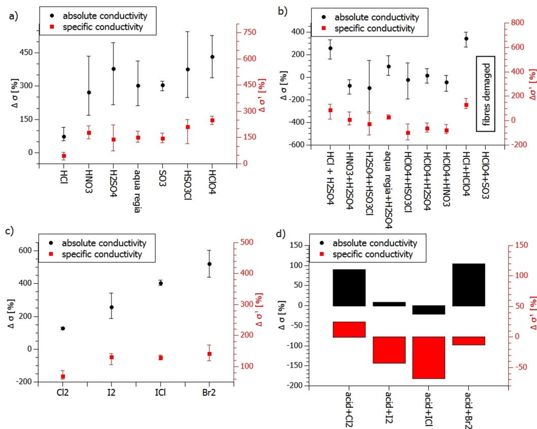
Figure 2. (a) Average percentage change in conductivity of wires treated with strong acids, wires were purified and soaked in 60% H 2 O 2 before acid treatment (b) average percentage change in conductivity of wires treated with two strong acids-one after another (difference in conductivity compared to the conductivity after first acid treatment), wires purified and pre-treated with 60% H 2 O 2 beforehand; (c) average percentage conductivity change after halogenation (halogenation performed on purified fibres); (d) Average conductivity change after halogenation of CNT fibers pretreated with HClO 4 , after initial purification and H 2 O 2 treatment. Whiskers represent differences between maximum and minimum values obtained in a series of experiments conducted.
