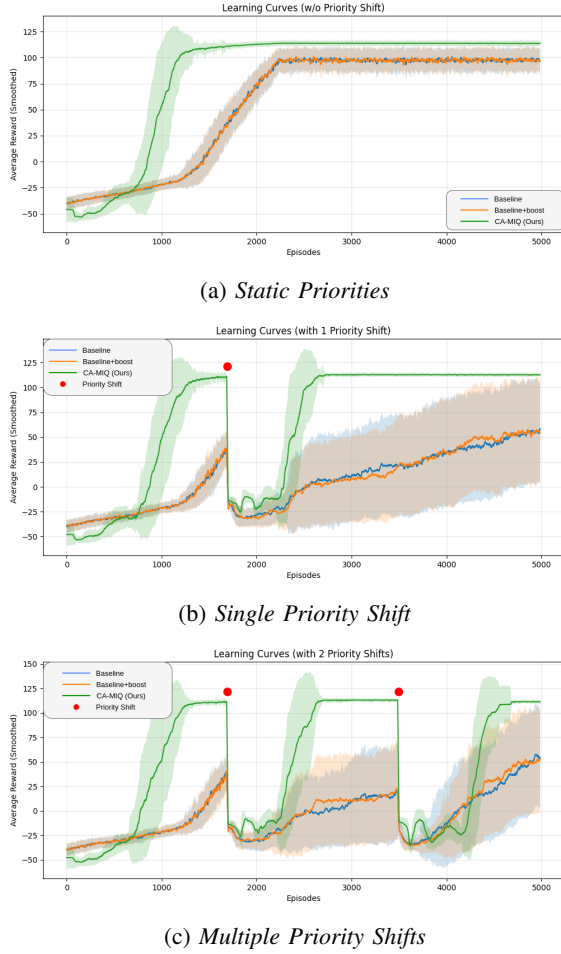
Fig. 2: Comparison of reward trends under static and dynamic conditions.
