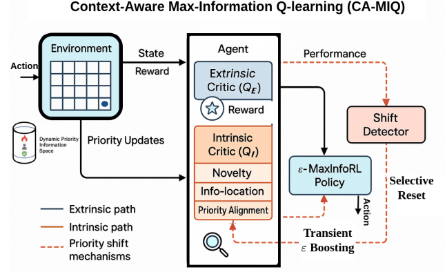
Fig. 1: CA-MIQ (Context-Aware Max-Information Q-learning) architecture. The environment supplies the current state to an agent equipped with two critics: an extrinsic critic Q^E that evaluates task reward-seeking behaviour (black path) and an intrinsic critic Q^I that aggregates novelty, information-location and priority-alignment signals (orange path). An \varepsilon -MaxInfoRL policy gate arbitrates between the critics to choose each action. A shift detector monitors performance; when a distributional change is detected it triggers a dashed orange priority-shift loop that transiently boosts exploration ( \varepsilon -boosting) and resets selectively the critics. Solid arrows denote data flow, whereas dashed arrows denote adaptive control signals.
