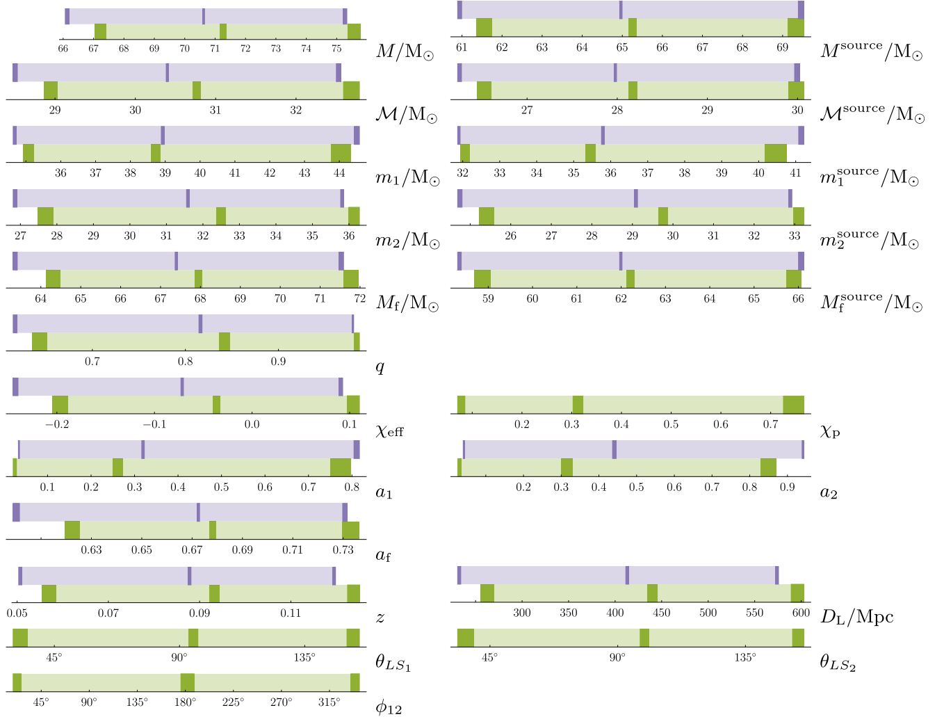
FIG. 9. Comparison of parameter estimates obtained by combining the nonprecessing-EOBNR and precessing-IMRPhenom models (as in Ref. [2]; light purple bars at the top) and by combining the precessing-EOBNR and precessing-IMRPhenom models (light green bars at the bottom). We show 90% credible intervals for selected GW150914 source parameters. The darker intervals represent uncertainty estimates for the 5%, 50%, and 95% quantiles (from left to right), as estimated by the Bayesian bootstrap.
