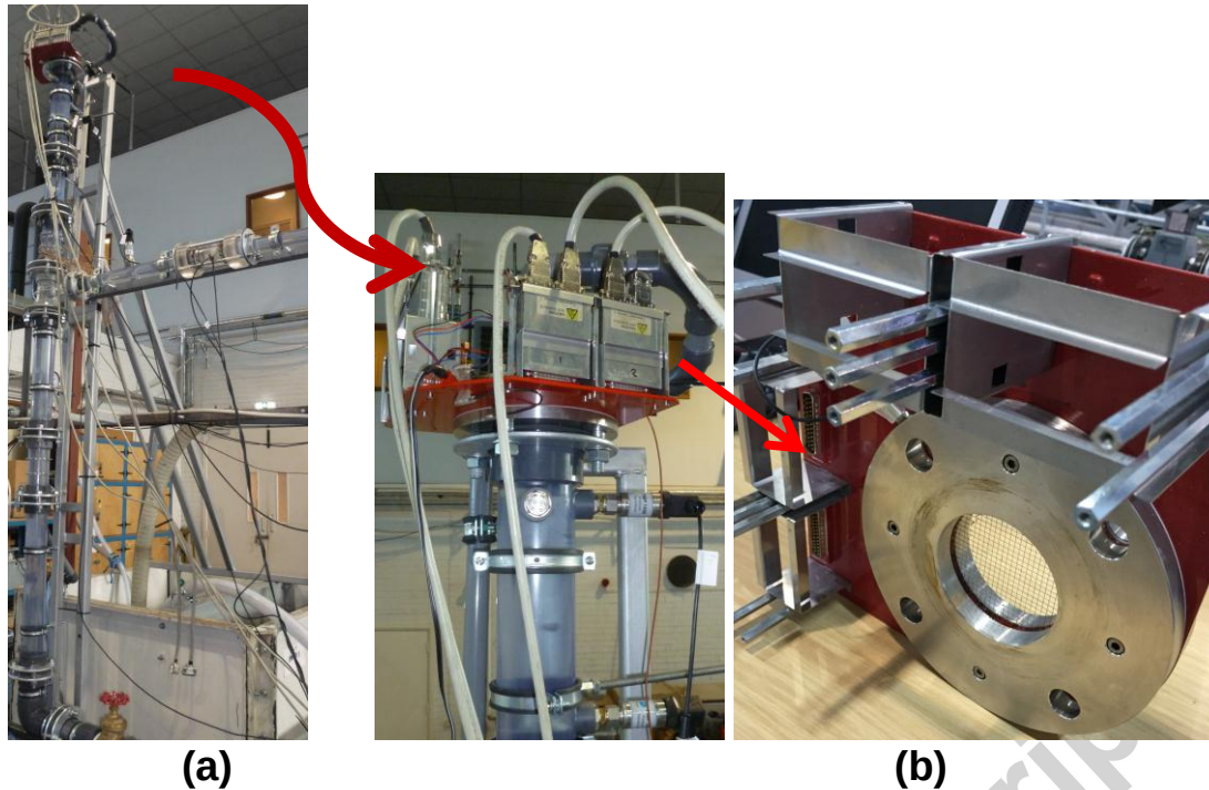
Figure 3(a) Gas-liquid pipe cyclonic separator with installed wire mesh sensor (b) Wire mesh sensor
