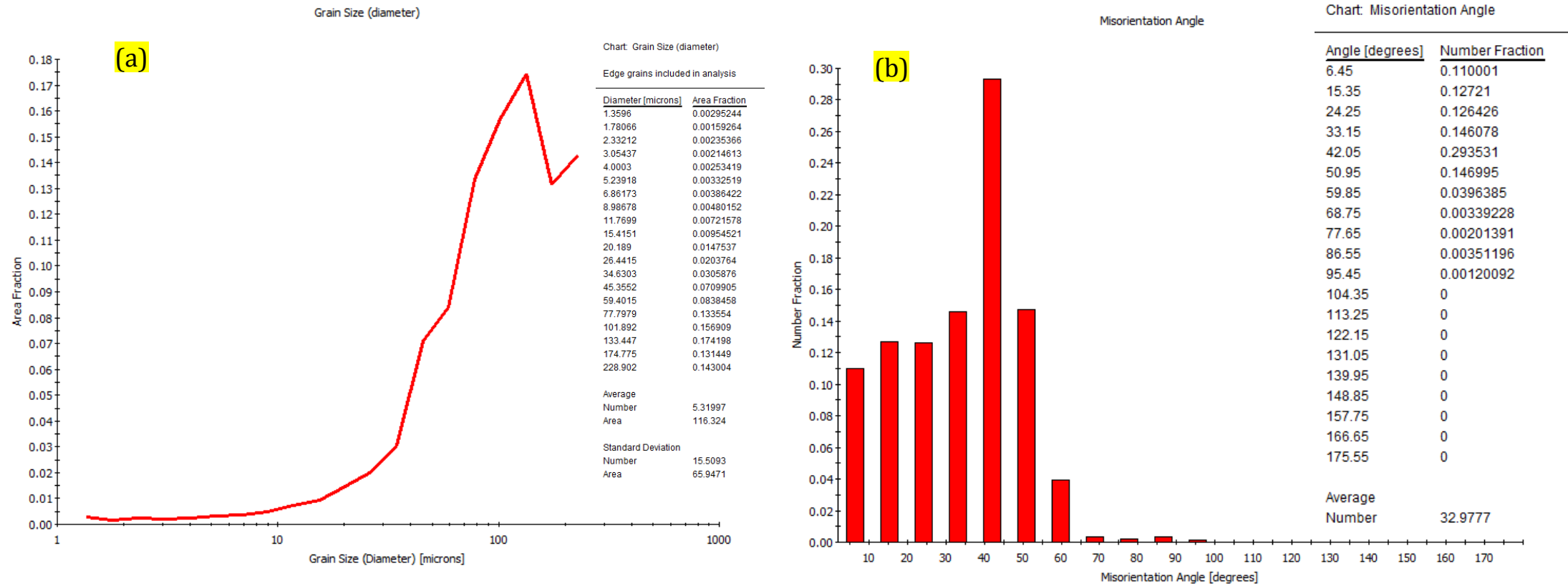
Fig. 6 EBSD analysis showing (a) average grain size and (b) misorientation angle distribution in the fusion region of EBW joints of Inconel 625 in the as-welded condition
