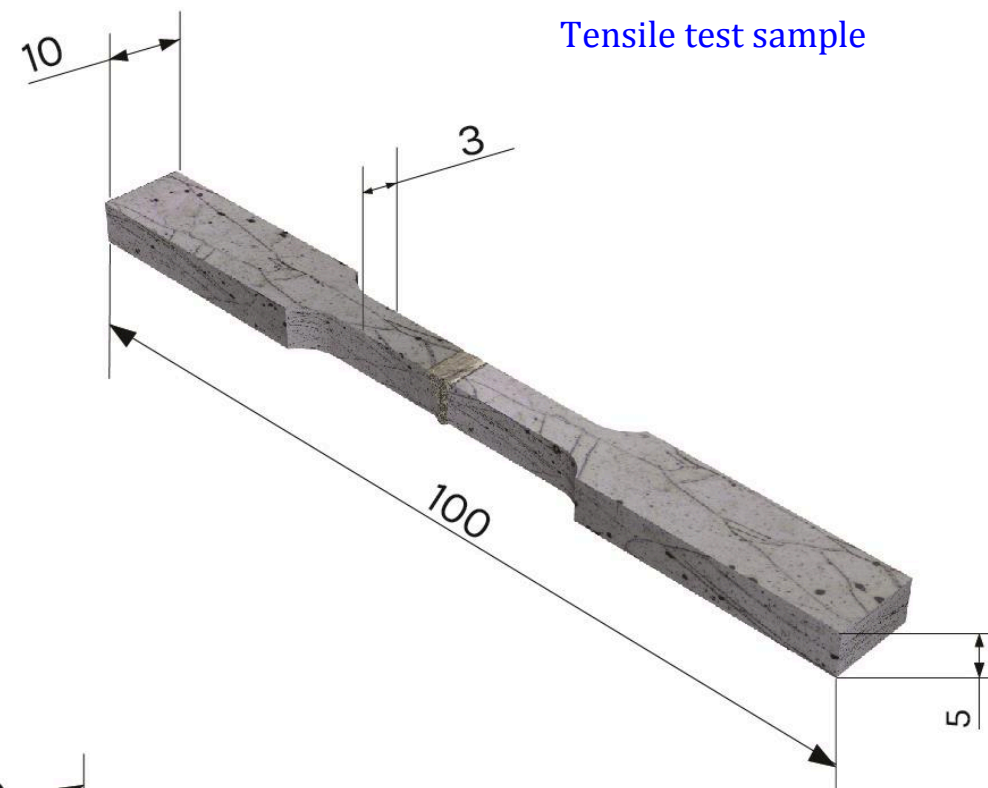
Fig. S1 CAD model depicting the samples extracted from EBW joints of Inconel 625 for analysing metallurgical and mechanical characteristics
