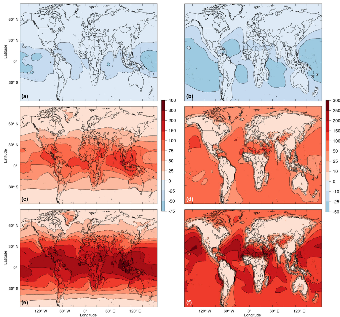
Figure 13. Annual mean changes in methanol abundances from run 1 ( \gamma = 0 , a, b ), run 2 ( \gamma = 0.2 , c, d ), and run 3 ( \gamma = 0.4 , e, f ), relative to the base run. Changes are shown in absolute (in pptv, a, c, e ) and relative terms (percentage change, b, d, f ).
