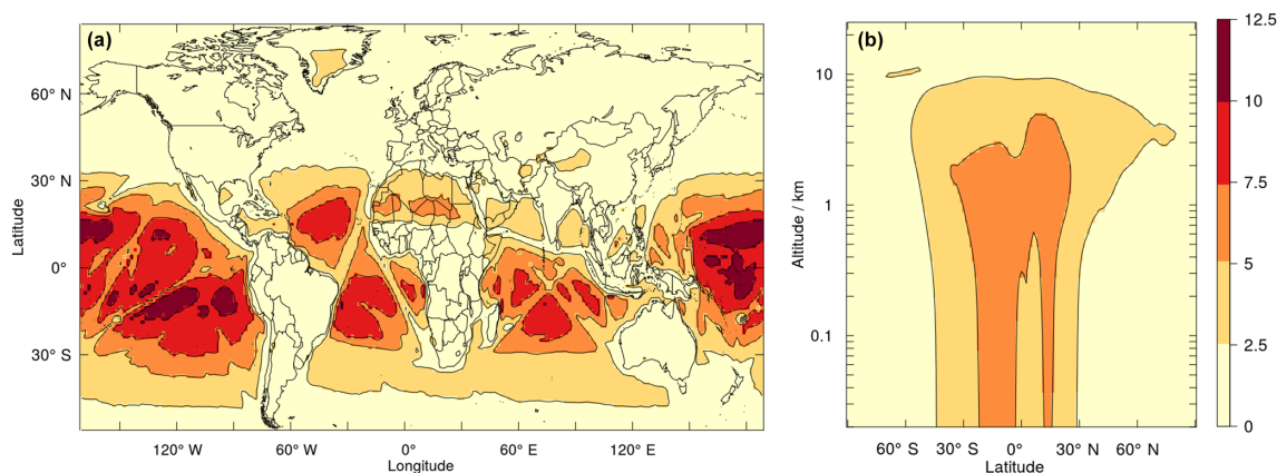
Figure 11. Annual mean percentage change in \text{HO}_2 concentrations from run 1 (relative to the base run) at the surface (a) and as a zonal mean (b).
