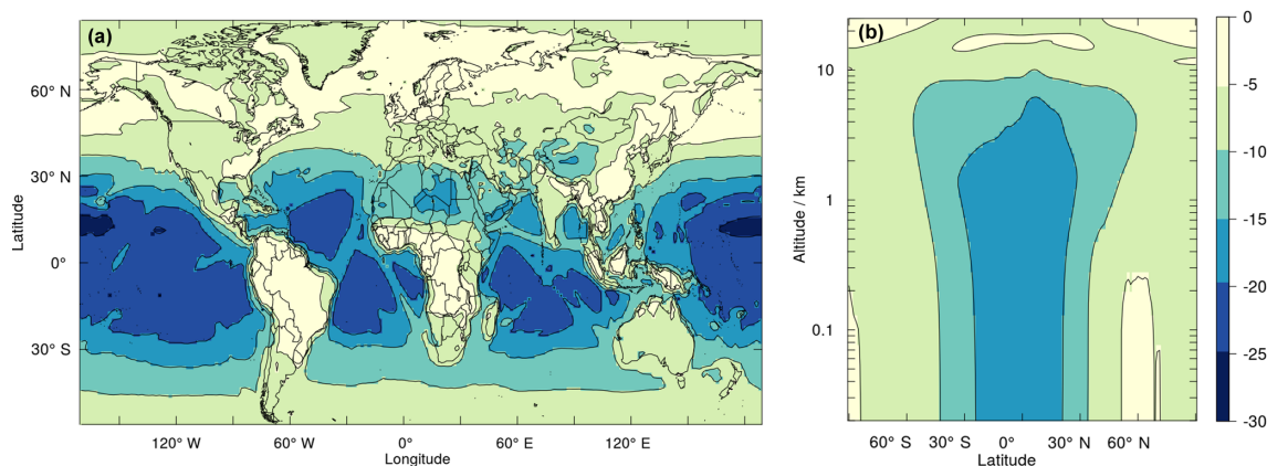
Figure 12. Annual mean percentage change in \text{CH}_3\text{O}_2 concentrations from run 1 (relative to the base run) at the surface (a) and as a zonal mean (b).
