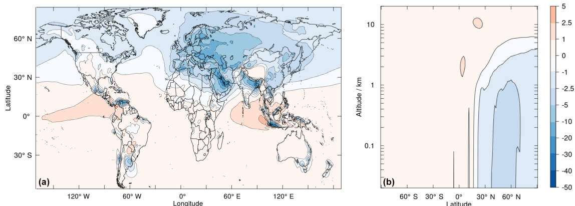
Figure 9. Annual mean percentage change in O 3 concentration at the surface (a) and as a zonal mean (b).
