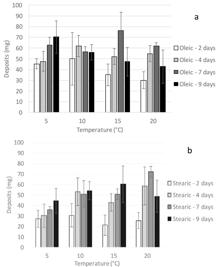
Figure 2. Average weight of FOG deposits during batch tests at the different temperatures for oleic solution (a) and stearic solution (b). Error bars indicate the standard deviation of the experimental results.
