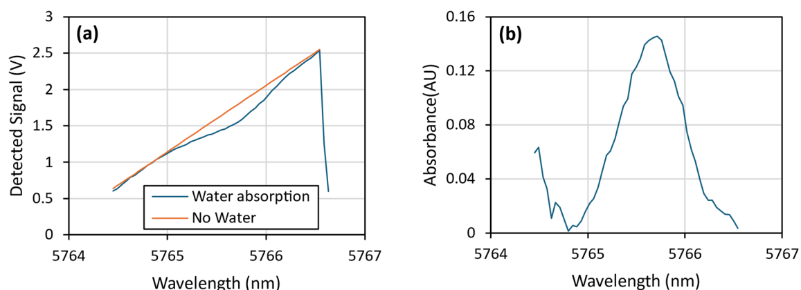
Fig. 3. (a) Received signals measured during a spectral scan created via a current ramp, measured in laboratory air using a pathlength of approximately 5 cm, and a nominally 5776 nm ( 1731\text{ cm}^{-1} ) QCL. The calculated absorbance (b) shows the presence of a water absorption line, confirmed to be at 5765.6 nm ( 1734.4\text{ cm}^{-1} ), as expected using the current and temperature tuning parameters of Fig. 2.
