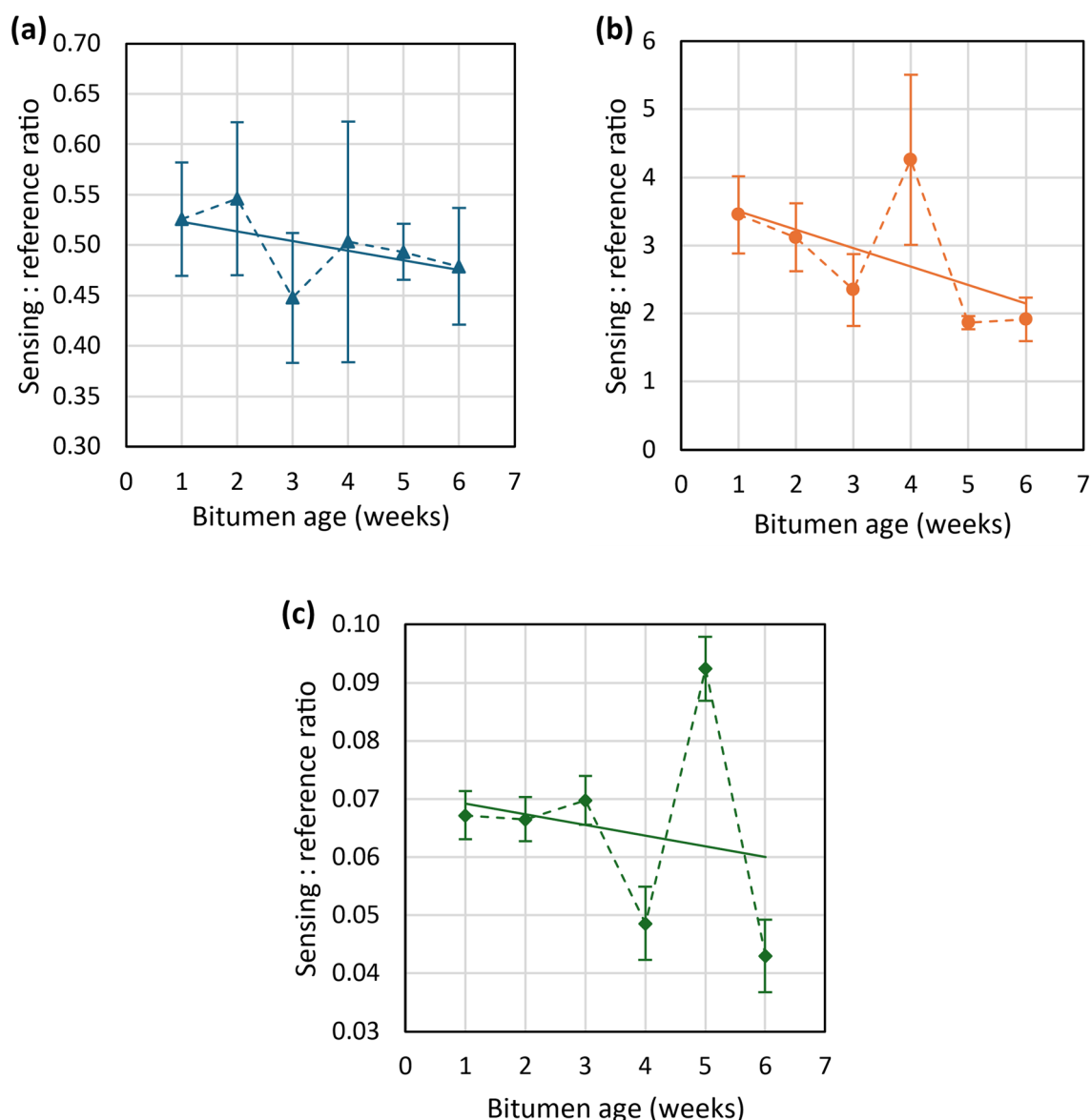
Fig. 12. 15° Diffuse reflection measurements of signal response of 1–6 week aged bitumen for (a) 5776 nm (1731 cm -1 ), (b) 6092 nm (1641 cm -1 ) and (c) 6277 nm (1593 cm -1 ).
