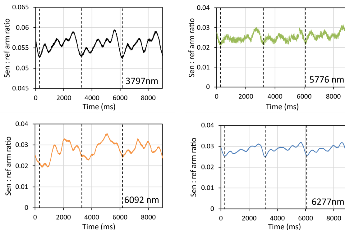
Fig. 17. Measurements for each laser showing variation in signal observed on a rotating sample of asphalt at a linear speed of 0.2 m/s. Vertical dashed lines indicate the start of a new cycle.
