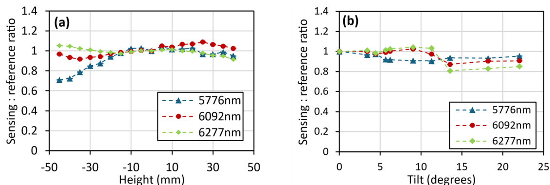
Fig. 9. (a) Instrument response to changes in the height of the measurement point and (b) response to changes in the angle of the sample at the measurement point for 15° diffuse geometry.
