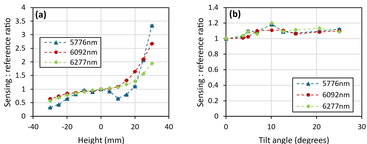
Fig. 8. (a) Instrument response to changes in the height of the measurement point (with increased y-axis scale to demonstrate parallax issue) and (b) response to changes in the angle of the sample at the measurement point, for 30° diffuse geometry.
