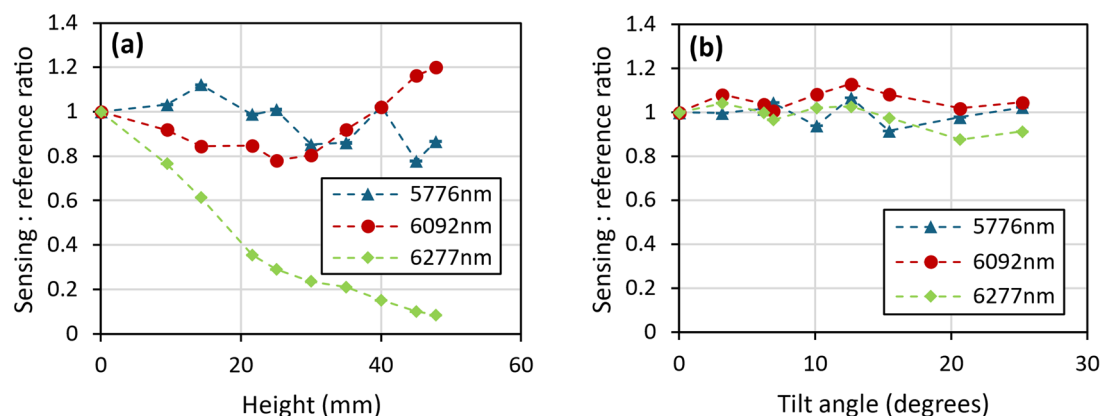
Fig. 7. (a) Instrument response to changes in the height of the measurement point, and (b) response to changes in the angle of the sample at the measurement point, both for the 15° specular geometry. Dashed lines between points are used as a guide to the eye.
