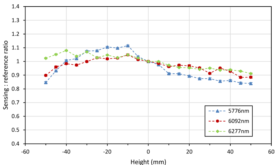
Fig. 19. Instruments response to changes in the height of the measurement point after being mounted onto the modified trolley.
