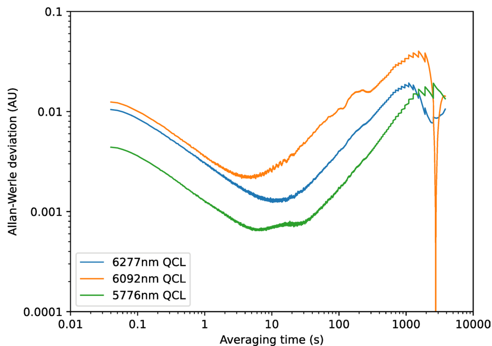
Fig. 22. Allan-Werle deviation measurement of 1-week UV-aged bitumen after being mounted onto the modified trolley.
