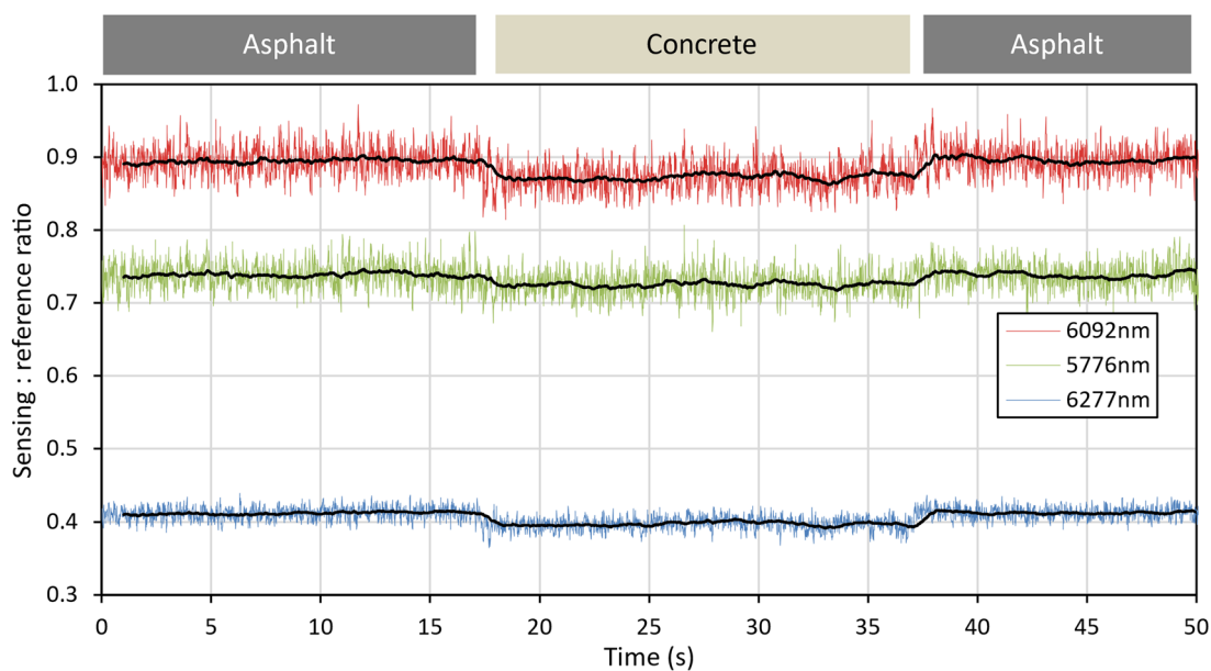
Fig. 25. Referenced QCL readings for measurements taken whilst transitioning between different surface materials. Black lines show a 1 s moving average.
