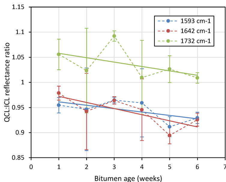
Fig. 14. Referenced signal response for averaged wavelength ranges corresponding to instrument measurement laser wavelengths for each bitumen sample.
