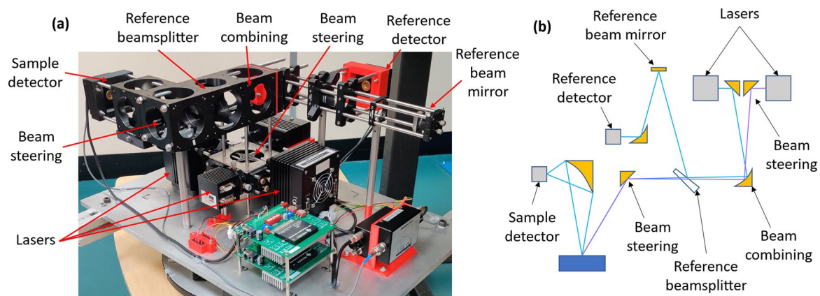
Fig. 5. (a) Photograph of the instrument (dimensions 600 × 400 × 240 mm) shown upside-down to demonstrate components, alongside (b) a 2D representation of the optical setup (2 lasers not shown are arranged above and below the plane of the drawing).
