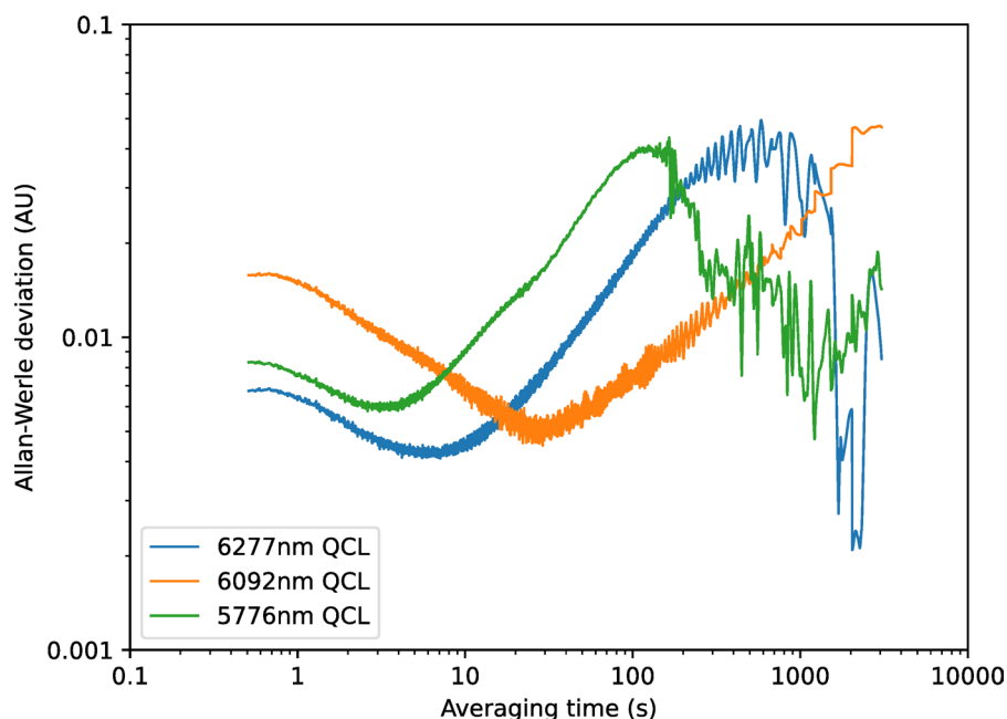
Fig. 15. Allan-Werle deviation for diffuse reflection measurements of an Infragold standard using referenced QCLs.
