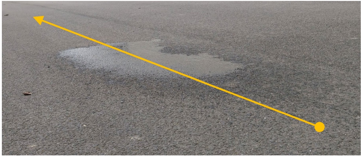
Fig. 26. Photograph of wet asphalt used to test instruments response to the presence of water, with arrow showing direction of travel. Regions of dry, damp and wet (shiny) asphalt can be seen.
