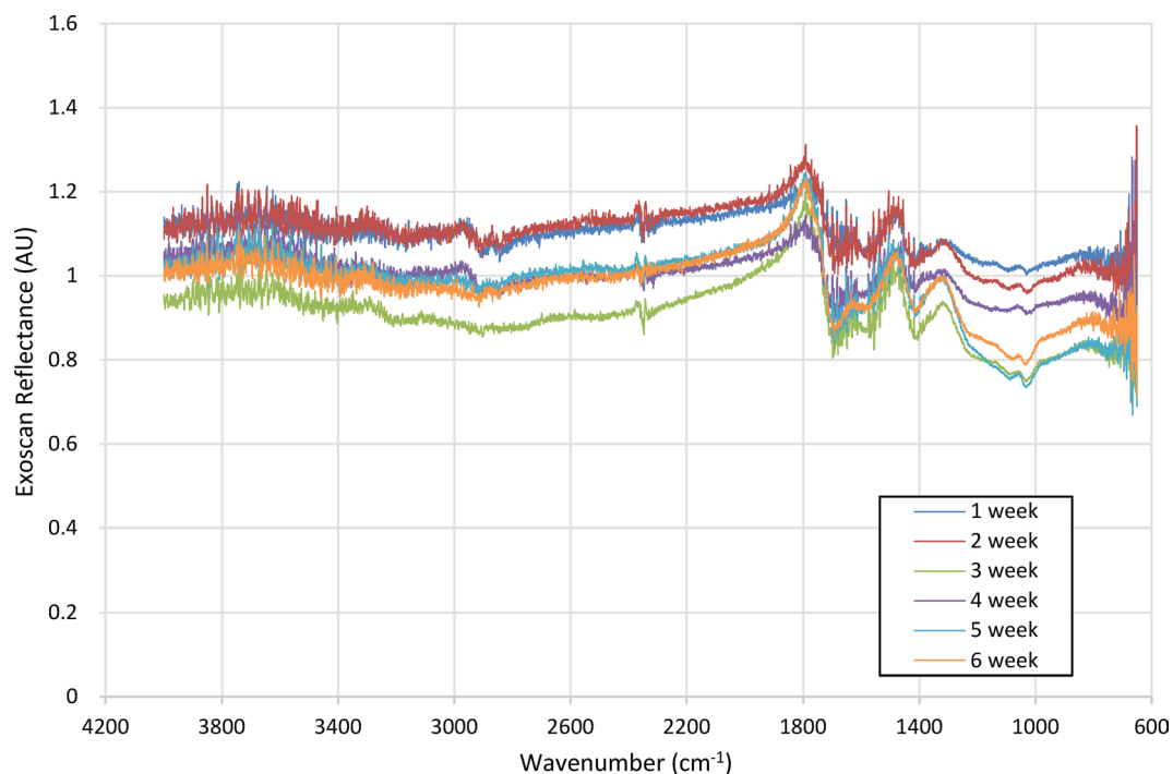
Fig. 13. Reflectance spectra taken of each bitumen sample using the Exoscan 4100 handheld spectrometer.
