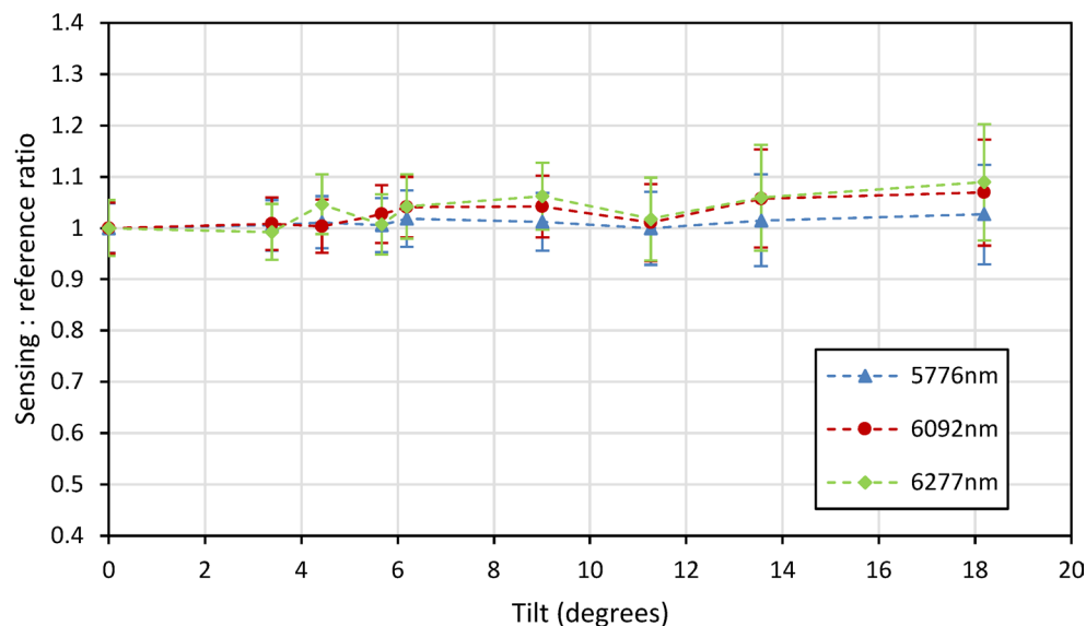
Fig. 20. Instruments response to changes in the angle of the sample at the measurement point after being mounted onto the modified trolley.
