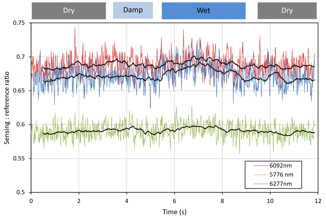
Fig. 27. Referenced QCL readings for measurements of response to wet asphalt. Black lines indicate a 0.5 s moving average.
