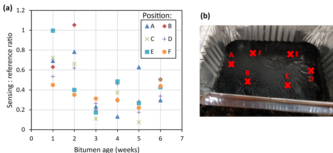
Fig. 11. (a) Example of difference between signals recorded at different locations on each bitumen sample for the 6092 nm ( 1641\text{ cm}^{-1} ) QCL and (b) the sensing locations on one of the bitumen samples.
