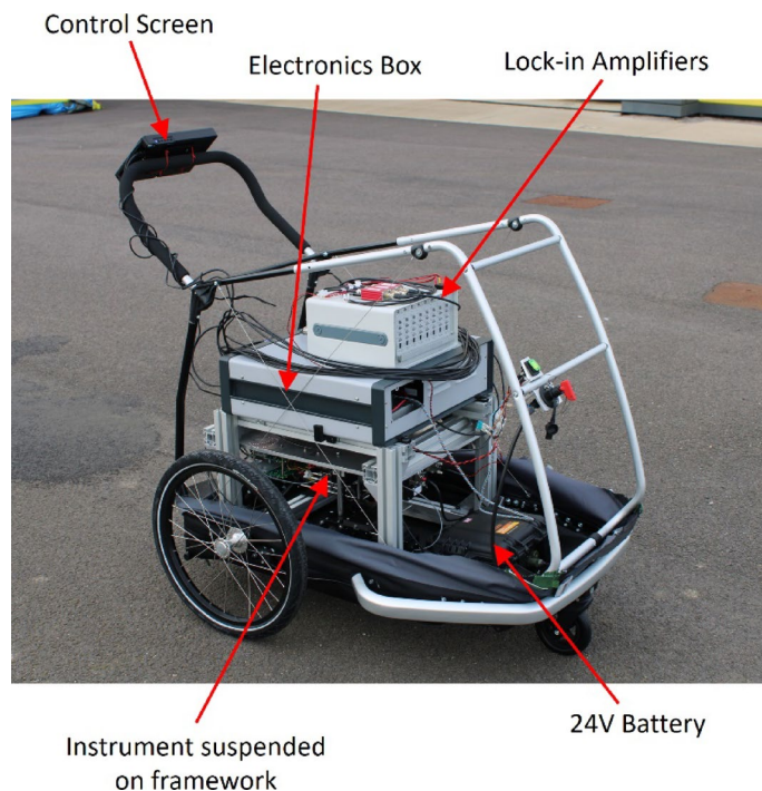
Fig. 18. Fully assembled instrument mounted onto modified trolley (dimensions 115 \times 86 \times 103 cm).
