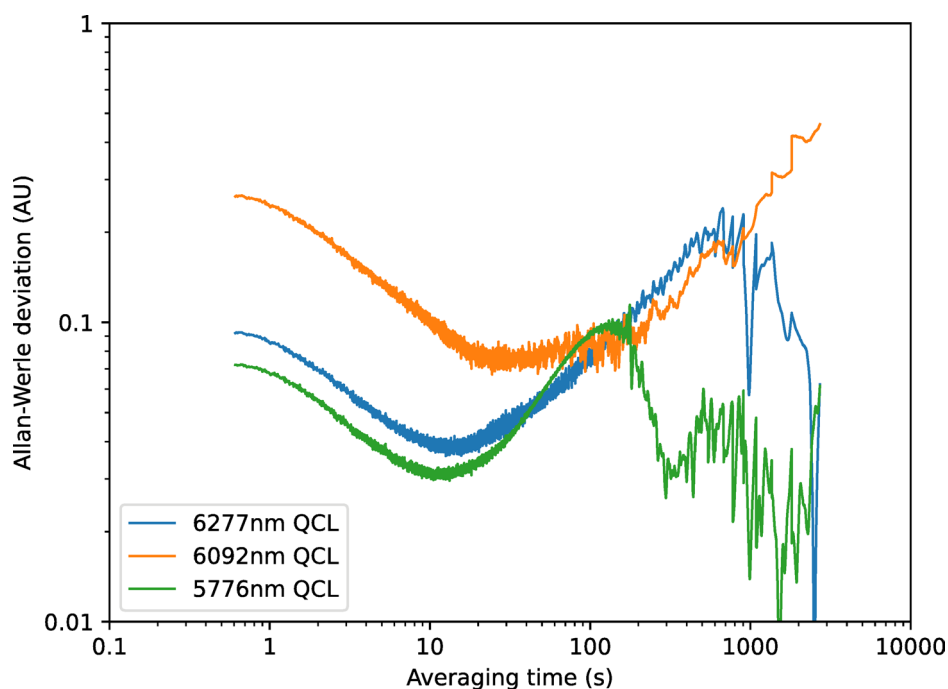
Fig. 16. Allan-Werle deviation for diffuse reflection measurements of 1-week UV-aged bitumen using referenced QCLs.
