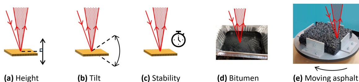
Fig. 6. Simplified illustration of instrument tests, shown here for a diffuse reflection geometry. Tests (a–c) were performed using a calibrated Infragold sample, whereas (d) and (e) were performed using bitumen and asphalt samples prepared as described in the text.
