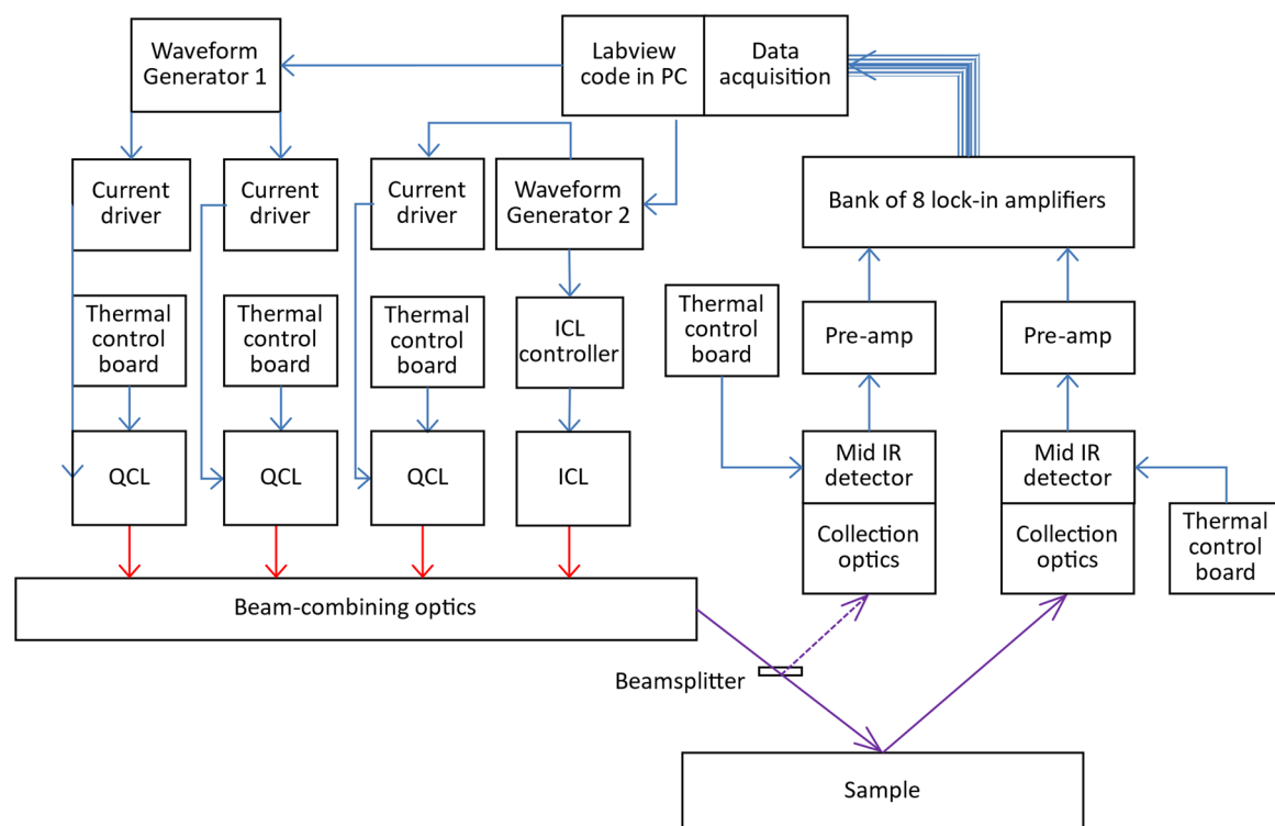
Fig. 4. Schematic diagram of the instrument system architecture.
