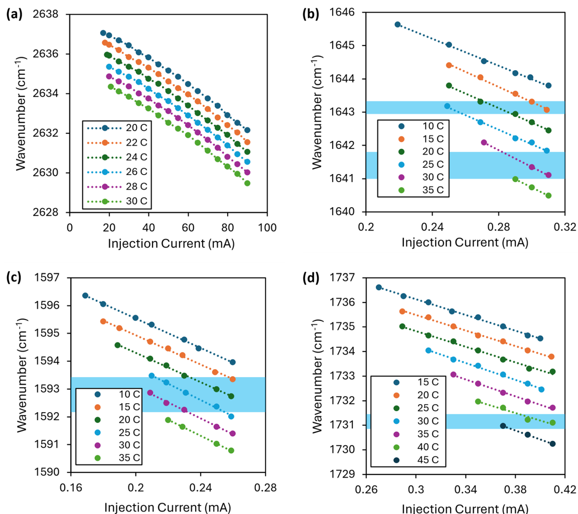
Fig. 2. Tuning characteristics of (a) the reference ICL and (b–d) the 3 measurement QCLs at different laser temperature setpoints. The shaded bars on the QCL graphs indicate the locations of the water absorption windows. The tuning curves illustrate the degree to which the width of the water windows limited the accessible level of current modulation.
