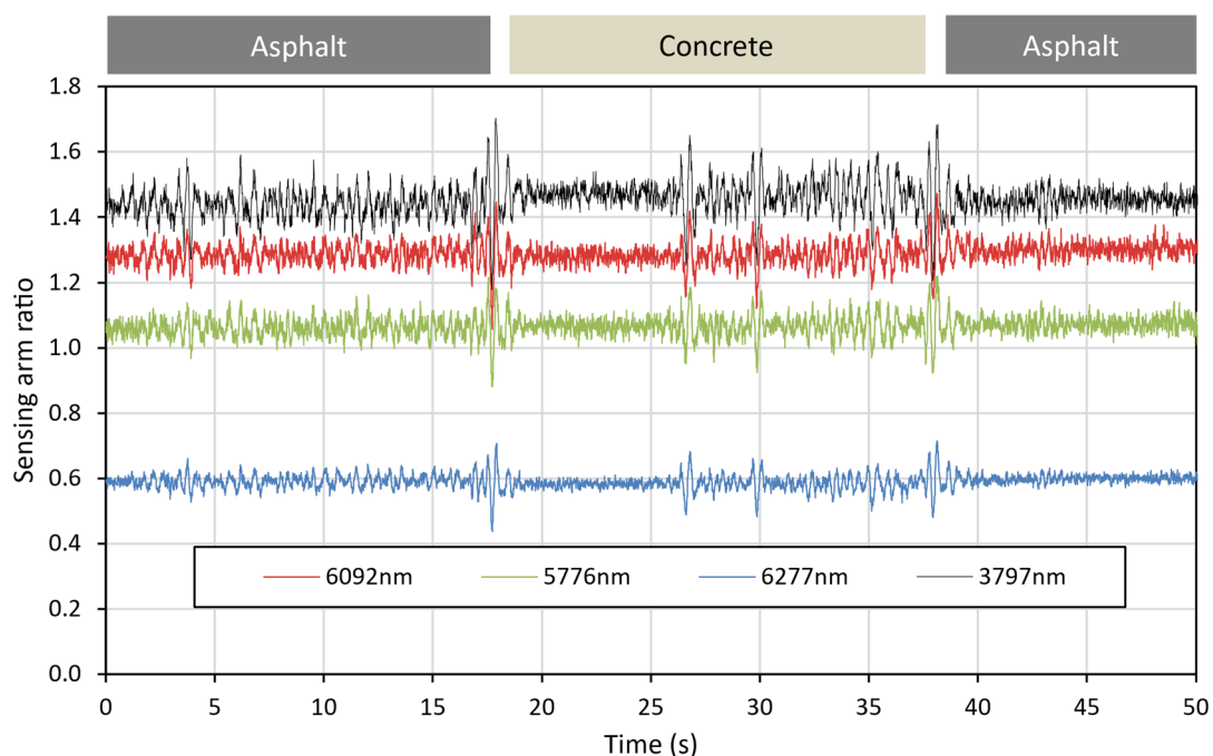
Fig. 24. Raw data (ratio of sensing arm to reference arm) for each laser whilst instrument was transitioning between different surface materials.
