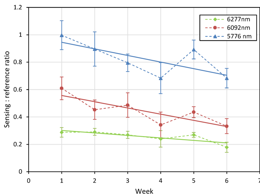
Fig. 21. Measurements of signal response of 1–6 week aged bitumen for each referenced QCL after being mounted onto the modified trolley. Solid lines show the trend in signal response for each laser with respect to bitumen age.
