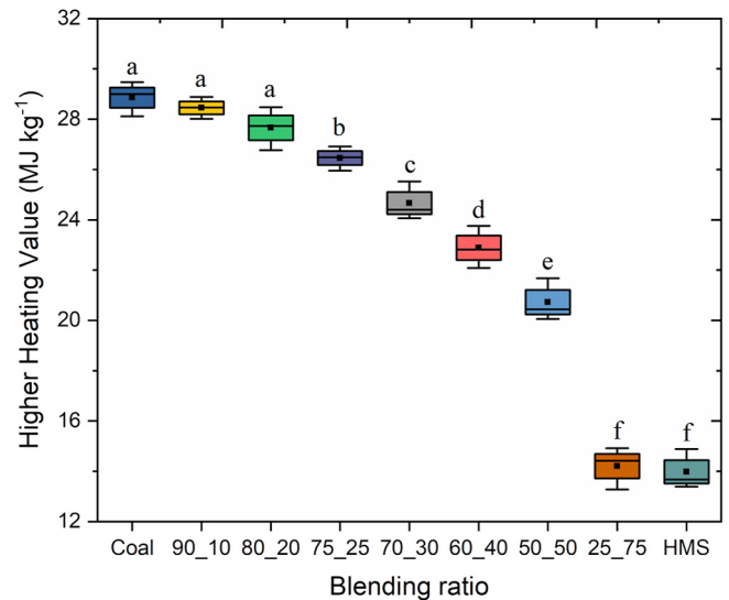
Fig. 8. Higher Heating Values of Coal and hydrochar blends.
