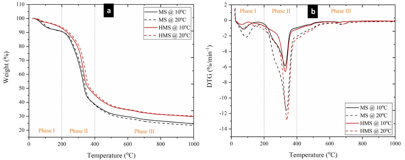
Fig. 7. a) Thermogravimetric (TGA) and b) Differential Thermogravimetric (DTG) curves of Spent Mushroom Substrate (MS) and its derived hydrochar (HMS).
