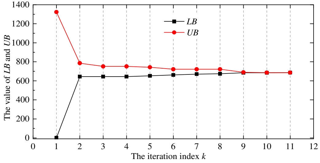
Fig.14-c The evolution of the value of LB and UB in case 10 for 135-node system
