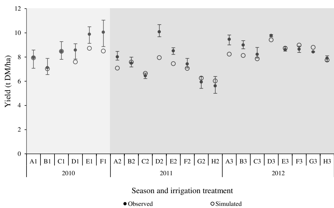
Figure 2 AquaCrop model simulated and observed brown onion ( cv. Arthur ) yield (t DM per ha) for selected irrigation treatments (Lacey and Ober, 2010; 2012) for the calibration (2010) and validation (2011-12) periods. Error bars show the maximum and minimum observations.
