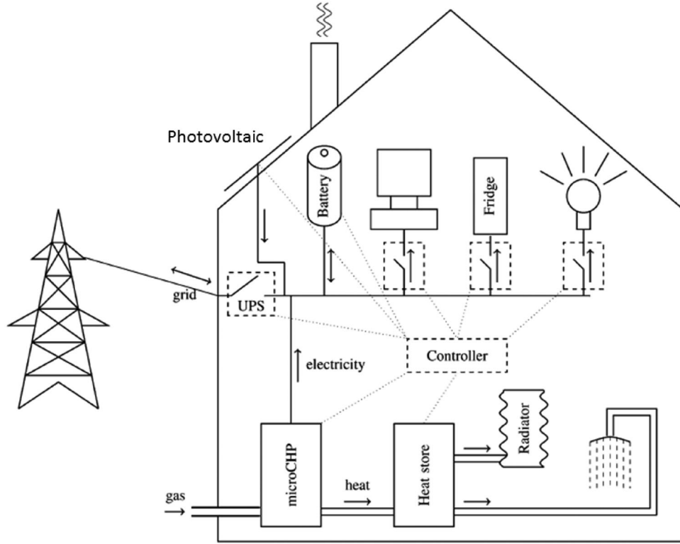
FIGURE 1. A model of home energy streams [27]: (i) Electricity supplies: the electricity grid, photovoltaic, micro CHP and UPS; (ii) Electricity demands (i.e., home appliances): television, fridge, light, radiator, shower, etc.; and (iii) Energy storage: battery.
