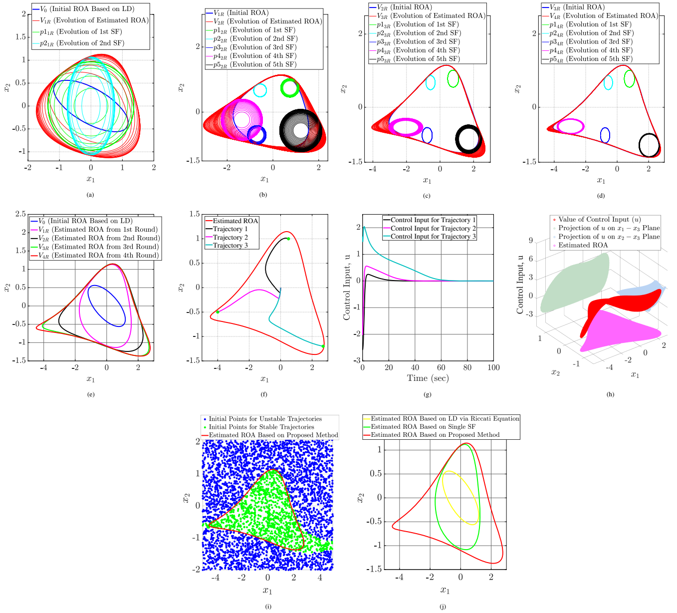
FIGURE 3 | Control System Design with ROA Estimation for Example 2. (a) ROA Estimation from the 1st Round, (b) ROA Estimation from the 2nd Round, (c) ROA Estimation from the 3rd Round, (d) ROA Estimation from the 4th Round, (e) Comparison of Estimated ROAs Across all the Rounds, (f) Trajectories of the System Under the Designed Control Law, (g) Control Input Responses for the Related Trajectories, (h) Value of Control Input within Estimated ROA, (i) Monte Carlo Simulation with Estimated ROA, (j) Comparison of Estimated ROAs Across Different Methods.
