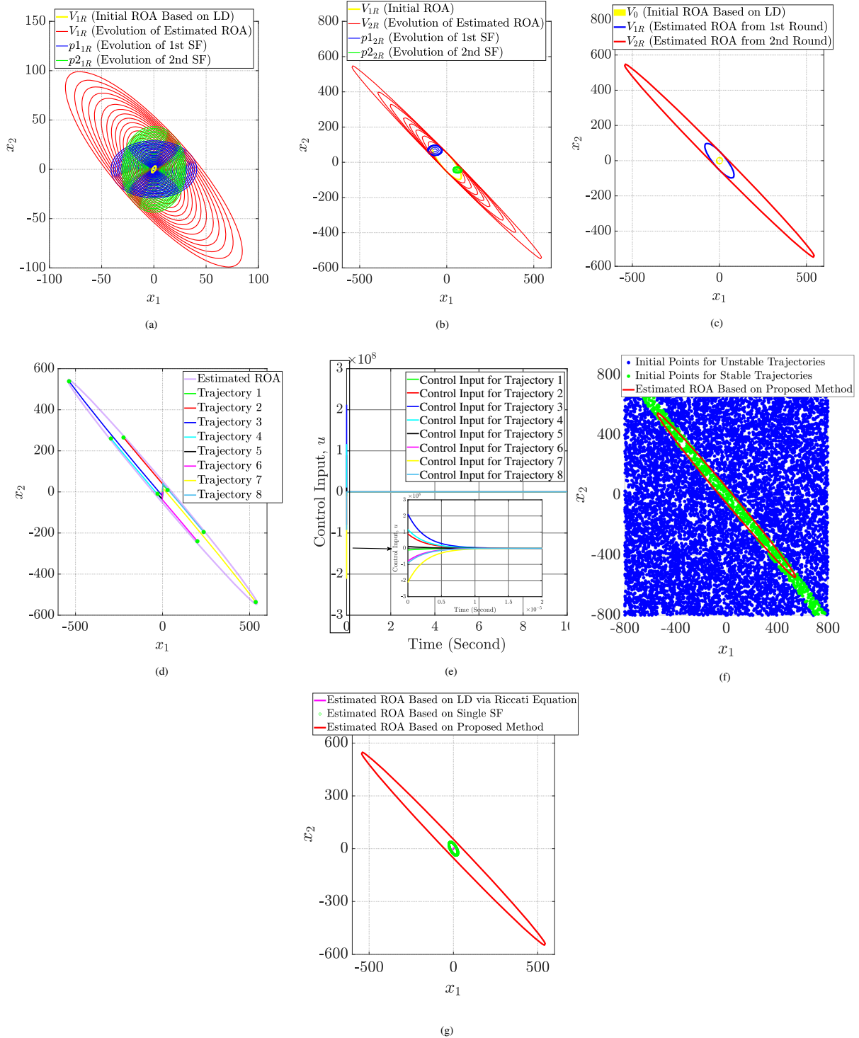
FIGURE 2 | Control System Design with ROA Estimation for Example 1. (a) ROA Estimation from the 1st Round, (b) ROA Estimation from the 2nd Round, (c) Comparison of Estimated ROAs Across all the Rounds, (d) Trajectories of the System Under the Designed Control Law, (e) Control Input Responses for the Related Trajectories, (f) Monte Carlo Simulation with Estimated ROA, (g) Comparison of Estimated ROAs Across Different Method.
