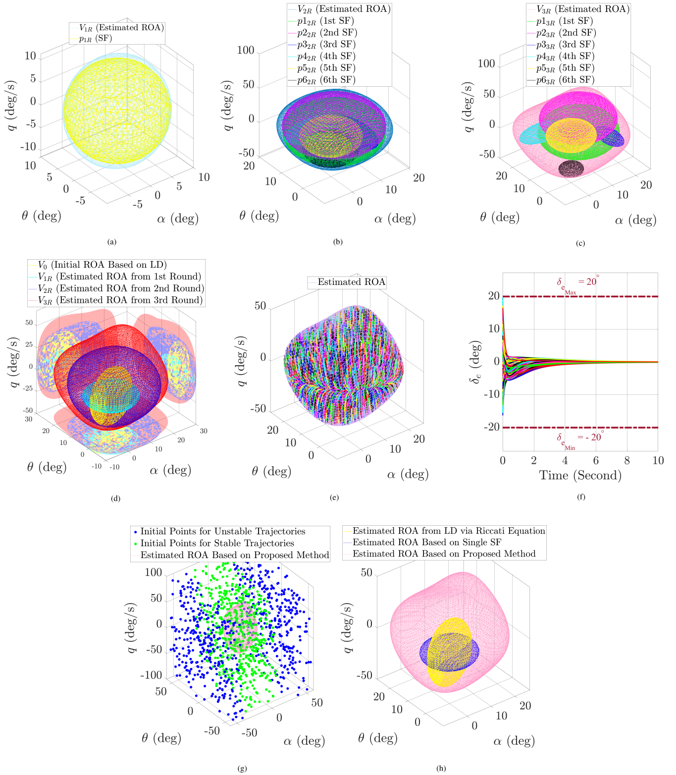
FIGURE 6 | Control System Design with ROA Estimation for Example 4: System with Both Control Input Saturation and State Constraints (Case II). (a) ROA Estimation from the 1st Round, (b) ROA Estimation from the 2nd Round, (c) ROA Estimation from the 3rd Round, (d) Comparison of Estimated ROAs Across all the Rounds, (e) Trajectories of the System Under the Designed Control Law, (f) Control Input Responses for the Related Trajectories, (g) Monte Carlo Simulation with Estimated ROA, (h) Comparison of Estimated ROAs Across Different Methods.
