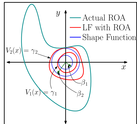
FIGURE 1 | Limitation of single SF based approach.
