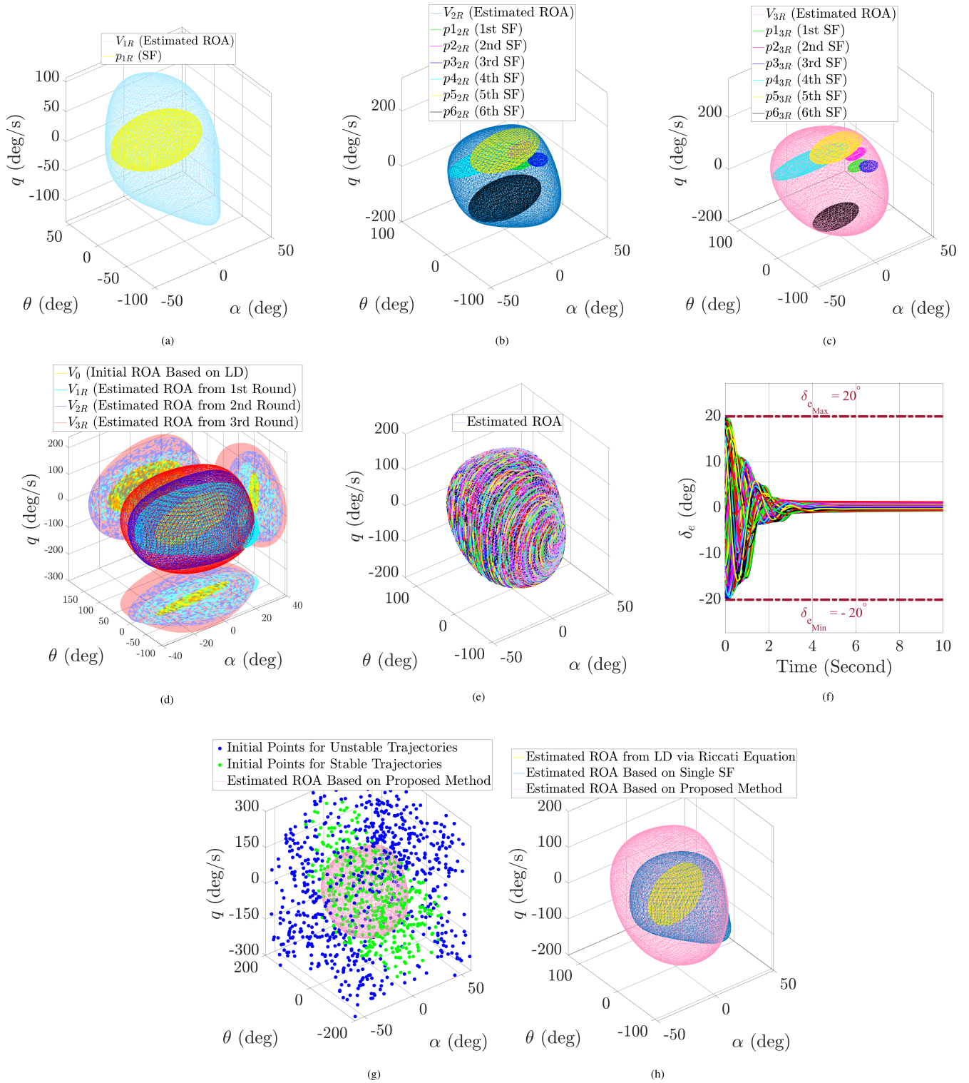
FIGURE 5 | Control System Design with ROA Estimation for Example 4: System with Control Input Saturation Only (Case I). (a) ROA Estimation from the 1st Round, (b) ROA Estimation from the 2nd Round, (c) ROA Estimation from the 3rd Round, (d) Comparison of Estimated ROAs Across all the Rounds, (e) Trajectories of the System Under the Designed Control Law, (f) Control Input Responses for the Related Trajectories, (g) Monte Carlo Simulation with Estimated ROA, (h) Comparison of Estimated ROAs Across Different Methods.
