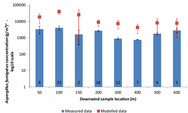
Fig. 2. Modelled and measured concentrations of A.fumigatus for (a) model calibration and (b) model validation. Graph A shows the modelled data at the start of the calibration process (initial model run) and at the end of the process (final model run). The measured data presented represent the arithmetic mean of the measured data at that particular downwind location. Error bars on the modelled (red) and measured (black) data denote minima and maxima. The numbers at the base of the measured data bars indicate the number of samples taken at that distance. 1 – Proxy for CFU/m 3 .
