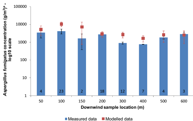
Fig. 4. Modelled and measured concentrations of A.fumigatus for the model validation after changes to the emission rate. Error bars denote minima and maxima for modelled (red) and measured (black) data. The numbers at the base of the measured data bars indicate the number of samples taken at that distance. 1 – Proxy for CFU/m³.
