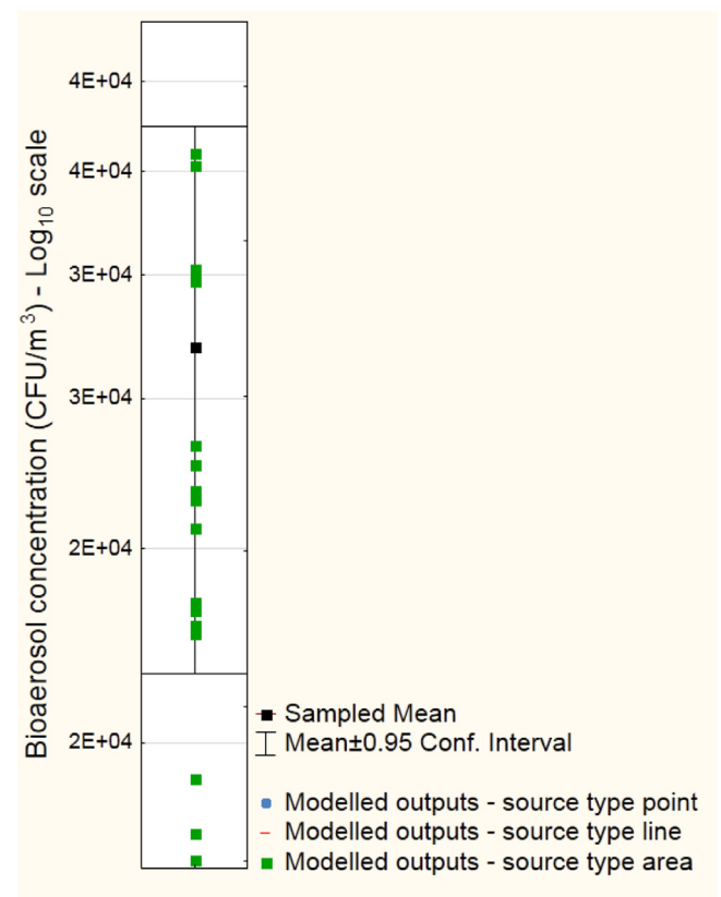
Fig. A1. Measured arithmetic mean (with a confidence interval of 95% from the sampled mean) and modelled output data generated from the SA at 10 m downwind.
