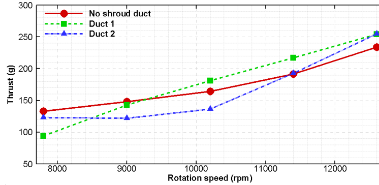
Figure 7 - Thrust produced at different rotation speeds by a single non-shrouded and shrouded propeller.
