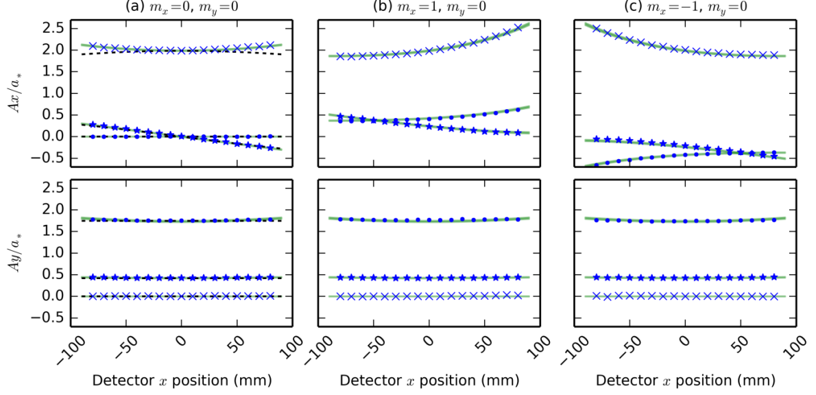
Figure 4. Comparison of translational scaling factors for \mathbf{S} = (0, -150, 265) mm and \mathbf{D} = (D_x, 0, 300) mm, for three surface gradients (a) m_x = m_y = 0 ; (b) m_x = +1, m_y = 0 and (c) m_x = -1, m_y = 0 . The top row shows the scaling factors for the speckle shift in the x direction ( A_x ) resulting from the object translations ( a_x, a_y and a_z ) while the bottom row shows scaling factors for the speckle shift in the y direction ( A_y ). The data points are the experimental results; ( \times ) A_{x,y}/a_x , ( \bullet ) A_{x,y}/a_y and ( \star ) A_{x,y}/a_z , and the dashed lines in (a) show the values predicted by the Yamaguchi's equations (for m_x = m_y = 0 ). The solid lines (green) are the values predicted by the extended equations presented in section 3. Here the thickness of the line denotes the minimum and maximum bounds predicted assuming an error in source and detector positions of \pm 1 mm in all directions.
