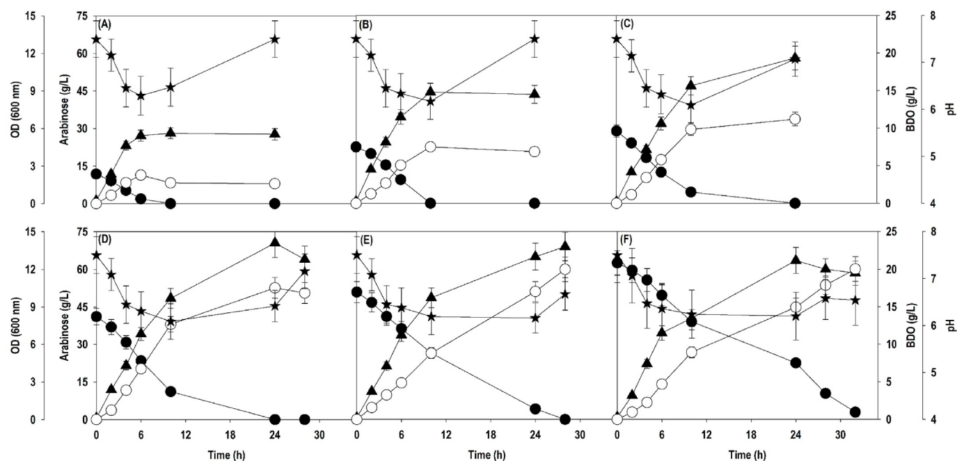
Fig. 1. Time course profiles for arabinose uptake, OD_{600} , BDO production and pH during shake flask cultivation at different levels of arabinose: (A) 10 g/L; (B) 20 g/L; (C) 30 g/L; (D) 40 g/L; (E) 50 g/L; (F) 60 g/L. Symbols: filled circle (arabinose), filled triangle ( OD_{600} ), empty circle (BDO) and filled star (pH).
