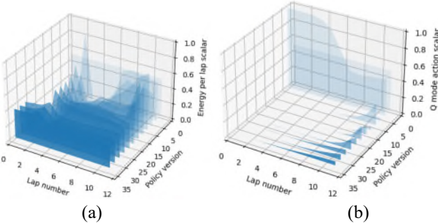
Fig. 3. Average continuous action scalars (a) Energy per lap; (b) Thermal management Q mode.
