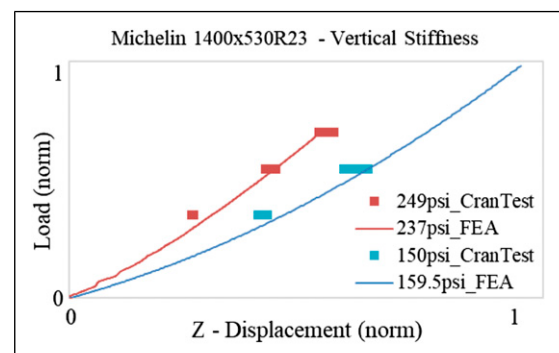
Figure 15. Vertical stiffness validation of Michelin 1400x530R23 comparing tests (CranTest) against FEA.
