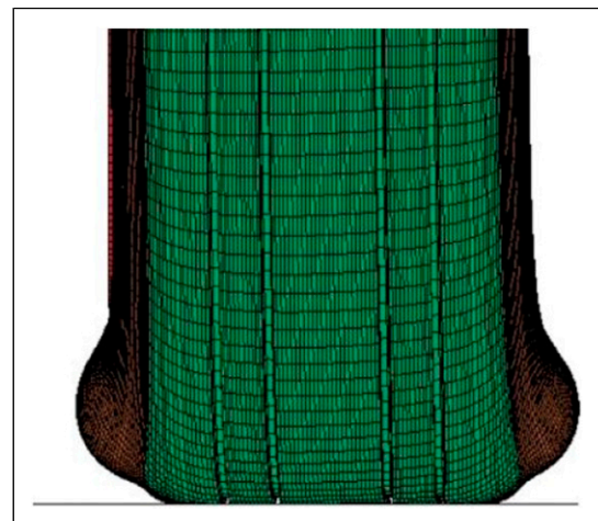
Figure 20. Representative Michelin 1400x530R23 un-yawed rolling with 59 kN vertical load at 237 psi and 20 mm initial lateral displacement.
