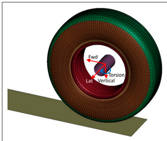
Figure 4. Tyre with loading directions.
