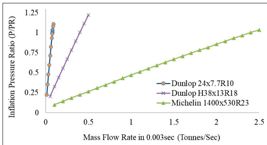
Figure 6. Mass air flow-rate variable for desired inflation pressure ratio (P/PR).
