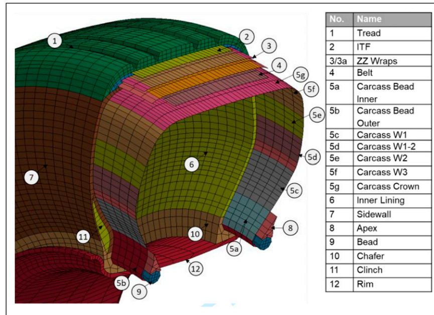
Figure 3. FEM segmentation into tyre components with variable V_f sidewall.
