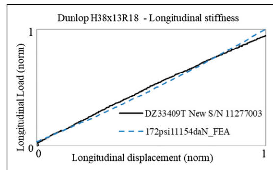
Figure 19. Representative longitudinal stiffness comparison for Dunlop H38x13R18 test results (S/N 11277003) against FEA.
