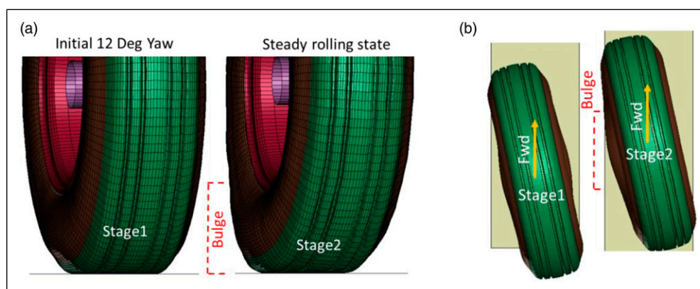
Figure 8. Stages of yawed tyre rolling conditions: (a) rear view and (b) top view.
