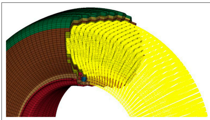
Figure 5. Internal segment set defining closed airbag control volume.
