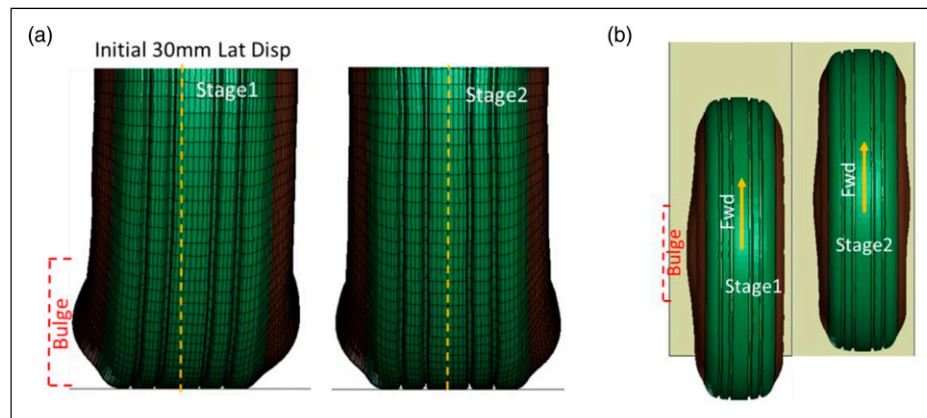
Figure 7. Stages of un-yawed tyre rolling conditions: (a) rear view and (b) top view.
