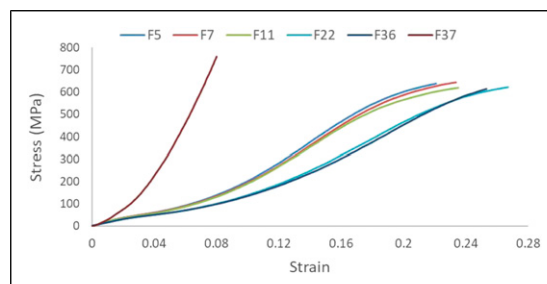
Figure 1. Uniaxial tensile test data for tyre reinforcement fabrics.
