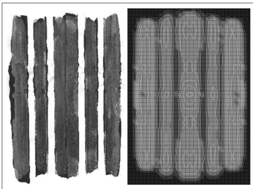
Figure 11. Footprint contact comparison for Dunlop 24x7.7R10 vertically loaded to 10.3 kN at 40 psi.
