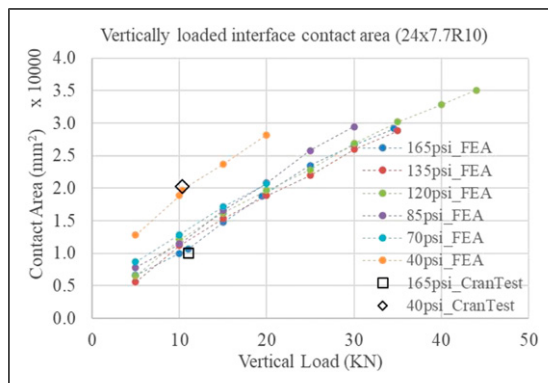
Figure 12. Footprint contact for vertically loaded Dunlop 24x7.7R10 comparing experimental (CranTest) and FEA.
