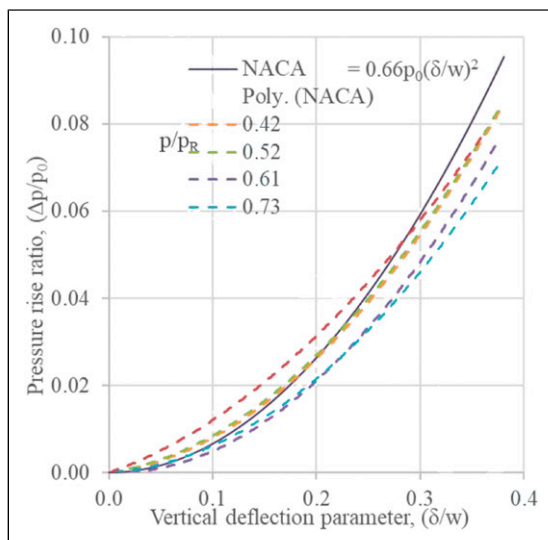
Figure 13. Pressure rise trends for Dunlop 24x7.7R10 against NACA 18 Type I tyres.
