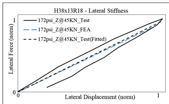
Figure 16. Lateral stiffness validation of Dunlop H38x13R18 for 45 kN vertical load inflated to 172 psi.
