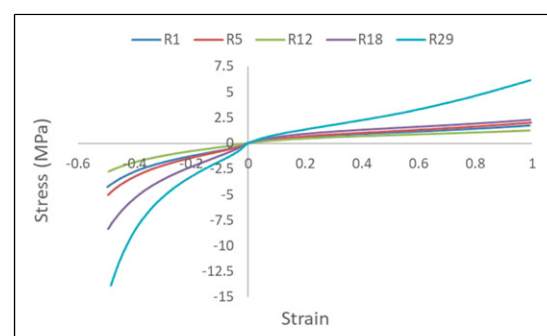
Figure 2. Uniaxial tensile and compression test data for tyre rubber compounds.
