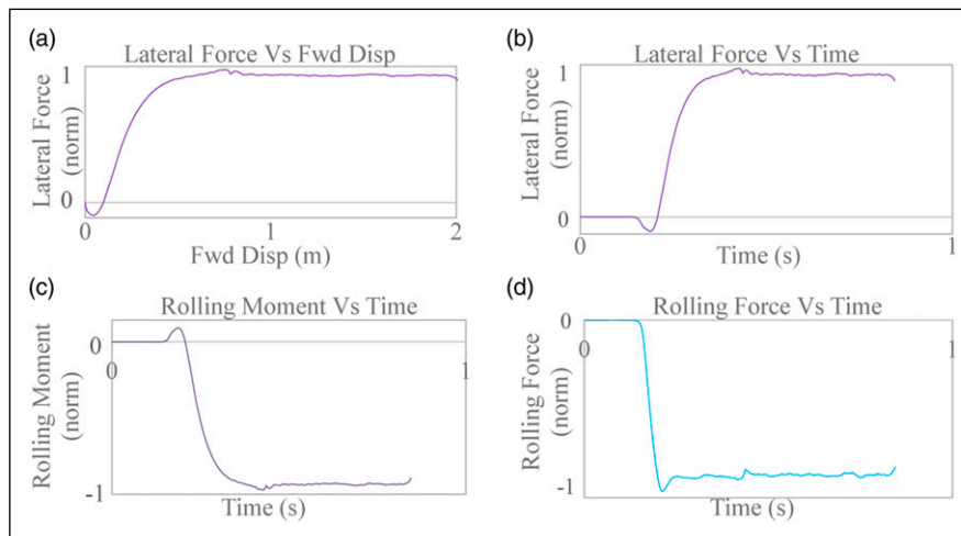
Figure 23. Representative Michelin 1400x530R23 yawed rolling with 59 kN vertical load at 237 psi and 8° yaw.
