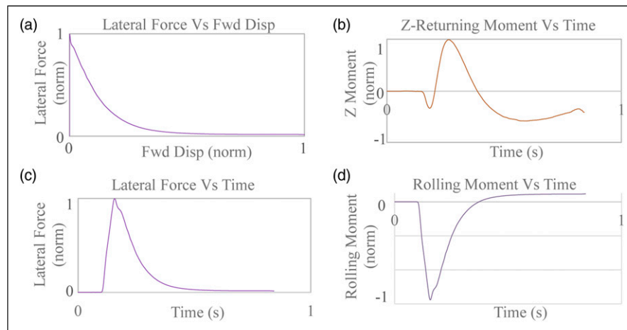
Figure 21. Representative Michelin I400x530R23 un-yawed rolling with 59 kN vertical load at 237 psi and 20 mm initial lateral displacement.
