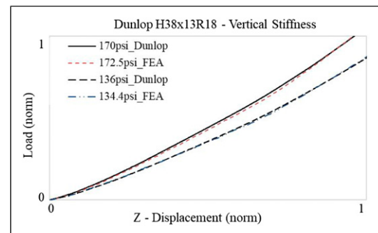
Figure 14. Vertical stiffness validation of Dunlop H38x13R18 comparing tests against FEA.
