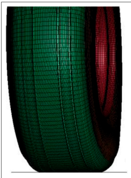
Figure 22. Representative Michelin I400x530R23 yawed rolling with 59 kN vertical load at 237 psi and 8° yaw.
