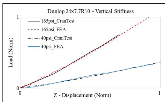
Figure 9. Vertical stiffness validation of Dunlop 24x7.7R10 comparing tests (CranTest) against FEA.
