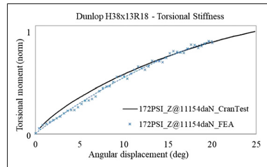
Figure 18. Representative Dunlop H38x13R18 torsional stiffness comparison of test results (CranTest) against FEA.
