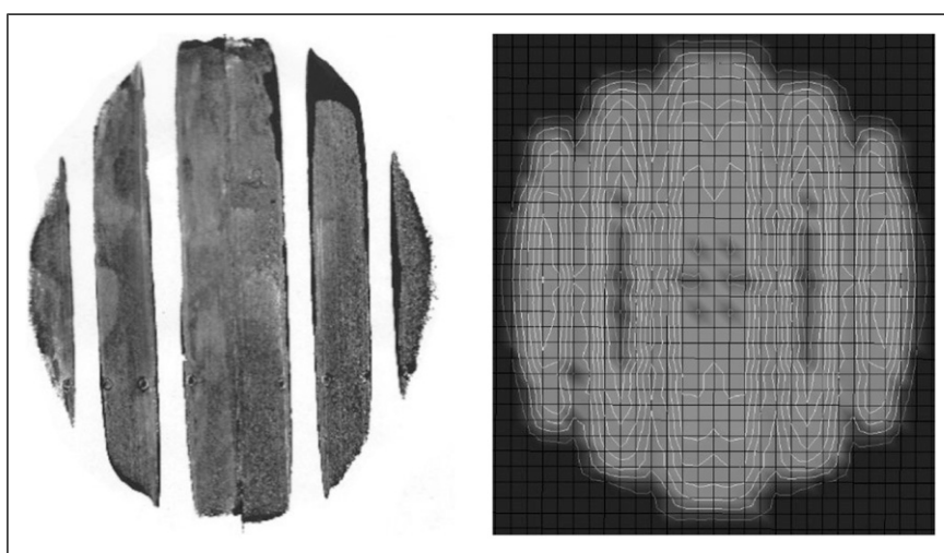
Figure 10. Footprint contact comparison for Dunlop 24x7.7R10 vertically loaded to 11 kN at 165 psi.
