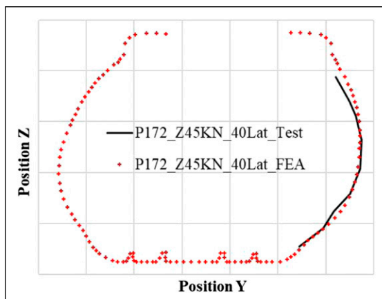
Figure 17. Representative FEA lateral bulge deformation (dotted line) comparison with scan measurements (continuous line) for Dunlop H38x13R18 with 45 kN vertical load at 172 psi.
