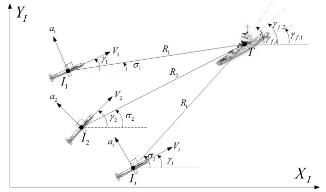
Fig. 1. Engagement kinematics for cooperative attacking of multiple interceptors.
