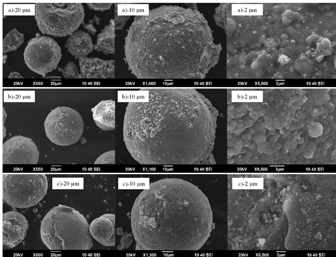
Fig. 10. SEM images of a) Mn 2 O 3 /FCC, b) hydrogen oxidation with Mn 2 O 3 /FCC at 300 °C (Mn 3 O 4 /FCC), and c) hydrogen oxidation with Mn 2 O 3 /FCC at 450 °C (MnO/FCC).
