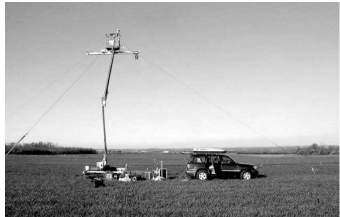
Fig. 7. Photograph of GB-SAR outdoor facility, with the linear scanner mounted on a 10-m-high hoist.
