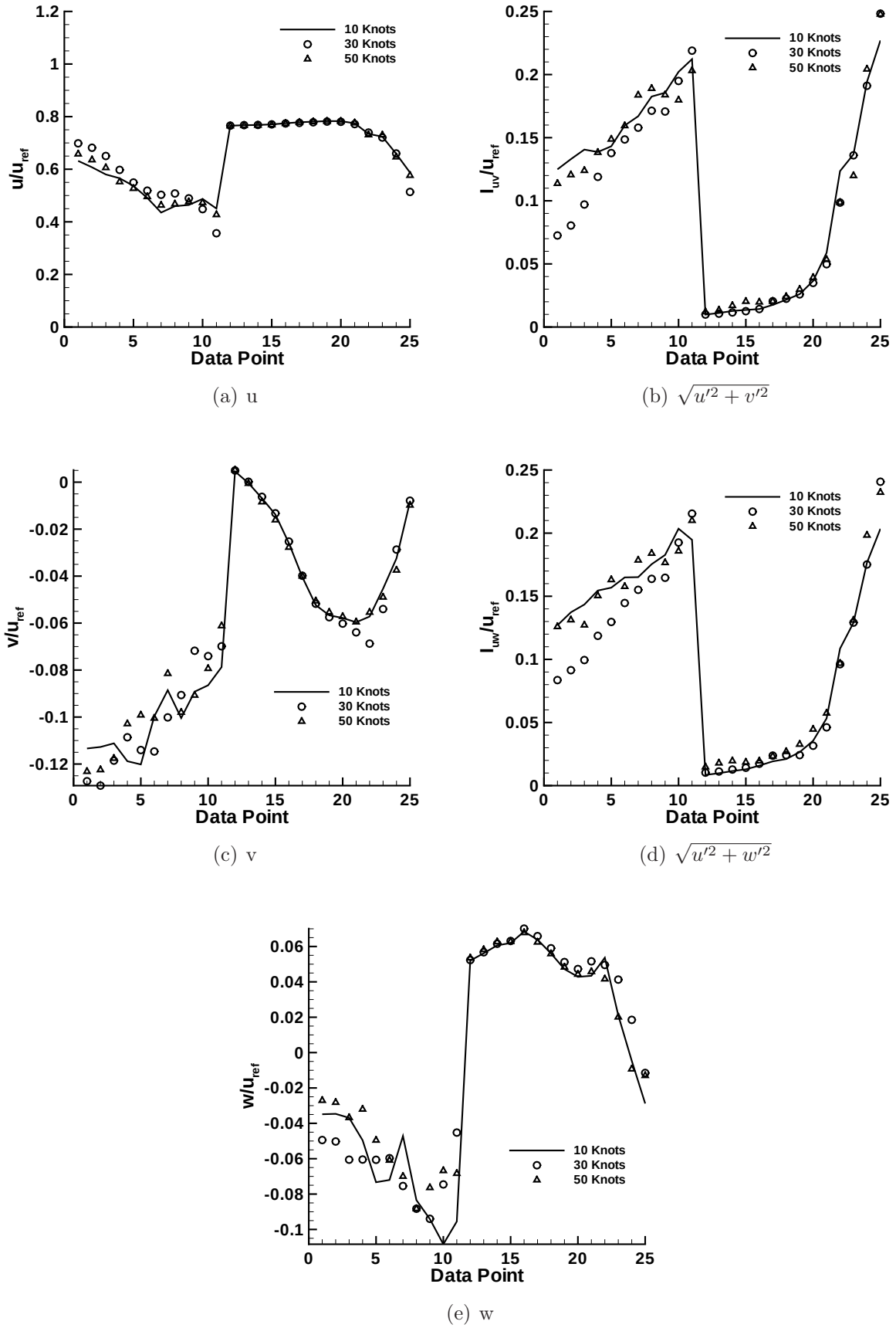
Figure 18. Flow properties taken at 25 points to test WOD velocity scaling. Note that points 12–21 are NOT the same as in the previous plots
