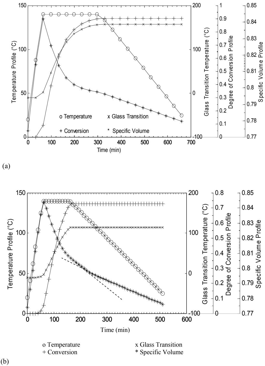
Fig. 11 Predicted property changes during two simulated representative thermal profiles
